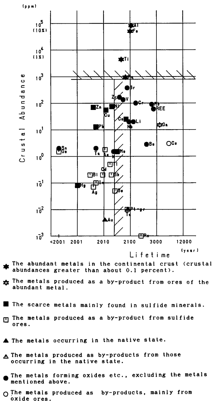
Fig. 1. Crustal abundances vs. static index since A.D. 2000.
