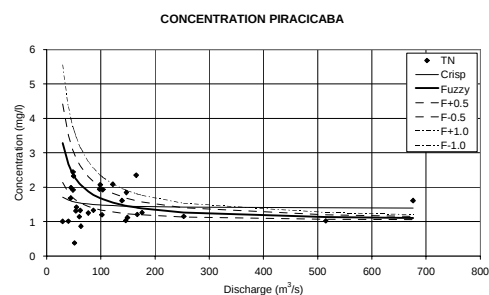
Fig. 5.4b TN concentration of Piracicaba River
