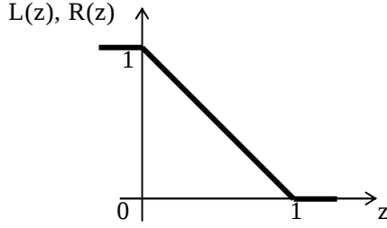
Fig. 5.1 Linear representation of L-R membership function for fuzzy numbers
