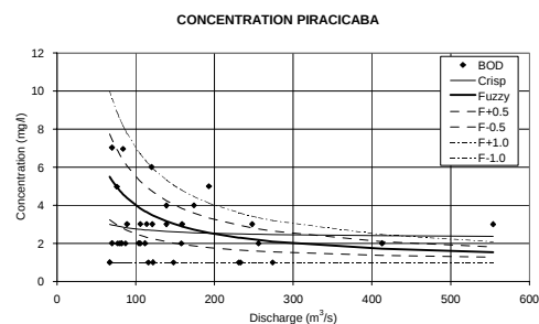
Fig. 5.4a BOD concentration of Piracicaba River
