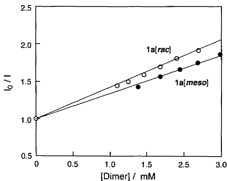
Figure 3. Stern-Volmer plots of the fluorescence quenching of ^*\text{Ru}(\text{bpy})_3^{2+} by (●) 1a[meso] and (O) 1a[rac] . Relative intensity ( I_0/I ) of the emission at 600 nm was measured in the presence of 10\ \mu\text{M} \text{Ru}(\text{bpy})_3^{2+} in deoxygenated phosphate buffer solution (10 mM, pH 7).
