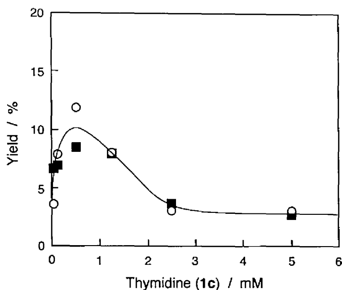
Figure 5. Influence of the concentration of thymidine ( 1c ) on the yields of C5–C5'-linked dihydrothymidine dimers (○, 3c[RS] ; ■, 3c[RR]+3c[SS] ) as observed at about 30% decomposition of 1c in the X-radiolysis of Ar-purged phosphate buffer solution (pH 7.0) containing sodium formate (200 mM).
