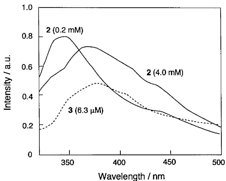
Figure 4. Fluorescence spectra of 2 (0.2 and 4.0 mM) and 3 (6.3 \mu M) in phosphate buffer at 293 K upon excitation at \lambda_{\text{ex}} = 270 nm.
