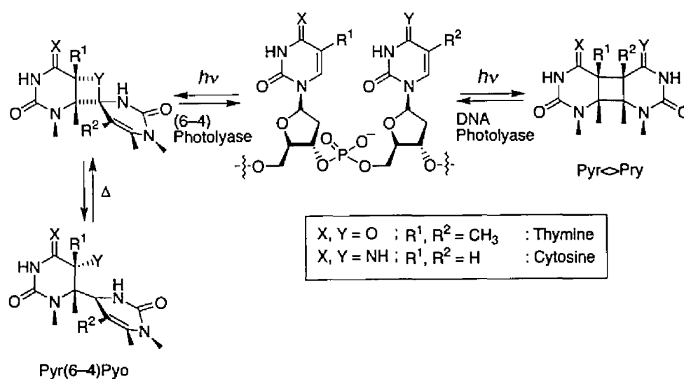
Figure 2. Photoproducts induced at dipyrimidine sites in DNA by UV radiation.
