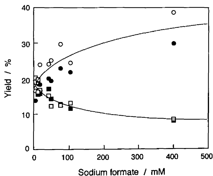
Figure 6. Variation of the yields of dihydrothymidines (●, 2c[S] ; ○, 2c[R] ) and C5–C5'-linked dihydrothymidine dimers (□, 3c[RS] ; ■, 3c[RR]+3c[SS] ) in the \gamma -irradiation (150 Gy) of Ar-purged phosphate buffer solutions (pH 7.0) of 1c (0.1 mM) with increasing concentrations of sodium formate.
