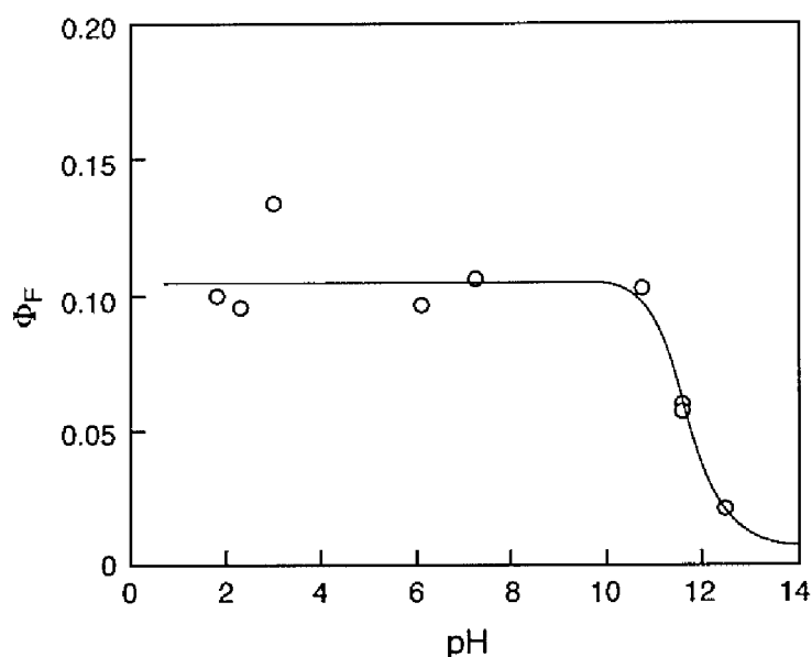
Figure 6. Titration curve monitored by the fluorescence quantum yield ( \Phi_F ) of 1a[meso] in phosphate buffer at 293 K. The half-equivalent point gave pK_a^* ( 1a[meso] ) = ~11.5.
