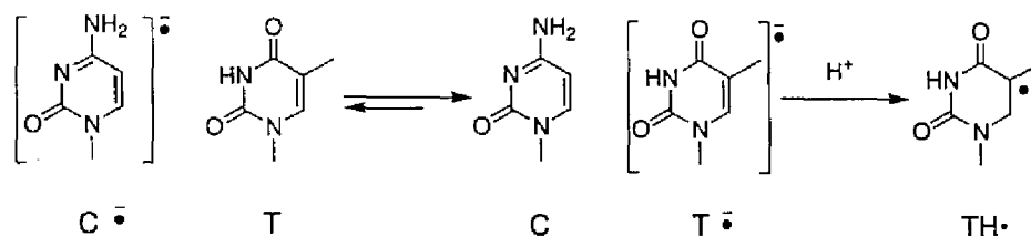
Figure 4. Mutual electron transfer process between cytosine and thymine.
