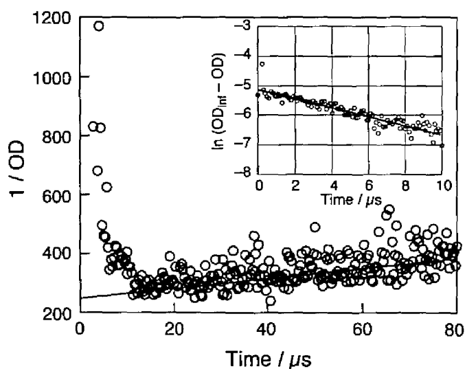
Figure 6. Pseudo-first order kinetics for the buildup component with absorbance at 400 nm in the 266-nm laser photolysis of \text{S}_2\text{O}_8^{2-} (50 mM) in phosphate buffer solution containing 1a [ meso ] (1.0 mM). The \text{OD}_{\text{inf}} corresponds to a plateau value of the absorbance at 400 nm due to the buildup component.
