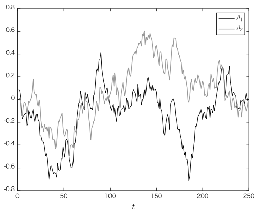
Figure 3: \rho = 0.5 の場合の \beta_t^1, \beta_t^2
