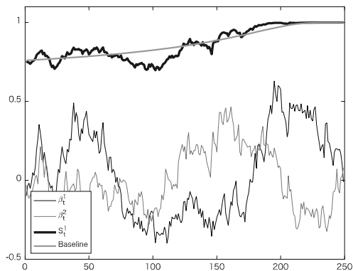
Figure 10: X_T(\omega) = x_1
