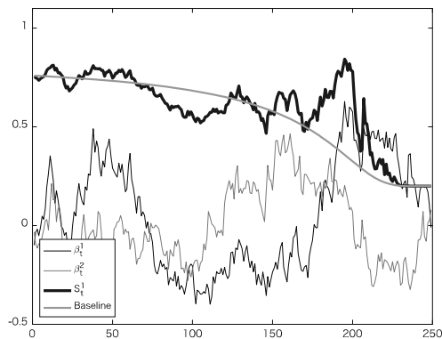
Figure 11: X_T(\omega) = x_0
