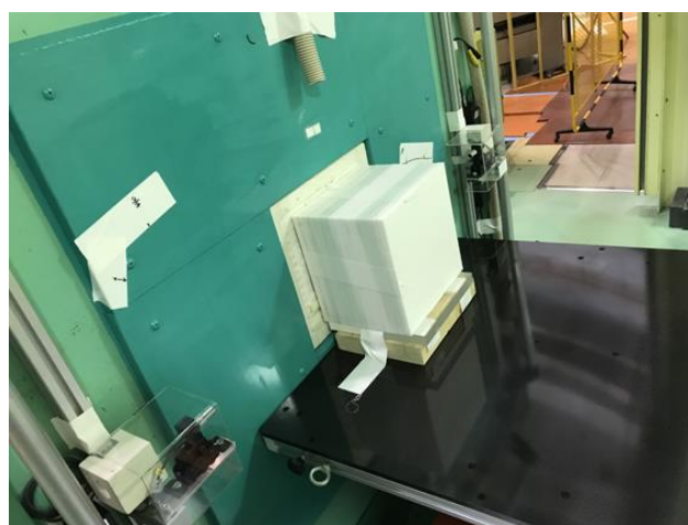
Fig. 1. The geometry of irradiation of RCFs by the KUR neutron source.
