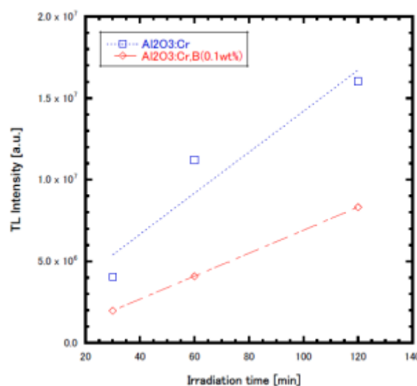
Fig. 2. Dose linearity for neutron and gamma mixed field of \text{Al}_2\text{O}_3 : 0.05 wt% Cr and \text{Al}_2\text{O}_3 : 0.05 wt% Cr, 0.1wt% B.
