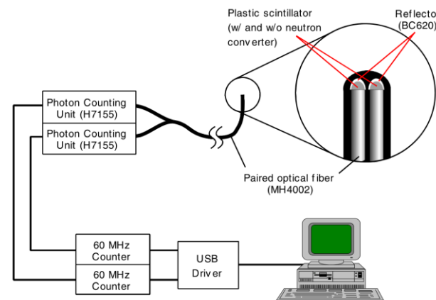
Fig. 1. Schematic illustration of SOF detector system. The SOF detector system consists of a small amount of plastic scintillator, a plastic optical fiber, a photo-multiplier tube, a charge pre-amplifier, a discriminator and a counter.
