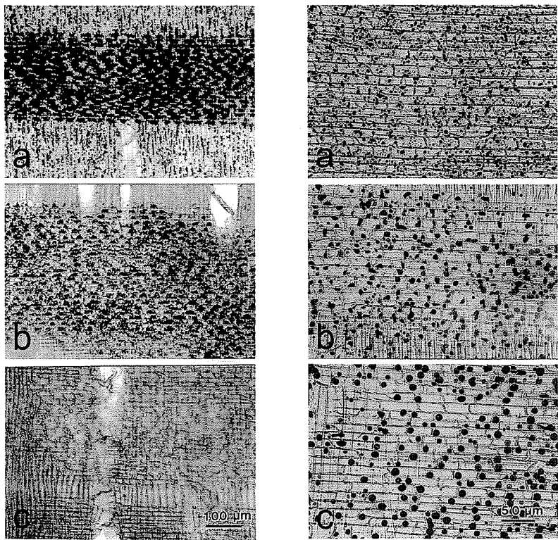
Photo 3 Light micrographs of radial longitudinal sections stained with iodine potassium. (a) Outer sapwood, (b) inner sapwood, (c) outer heartwood.
