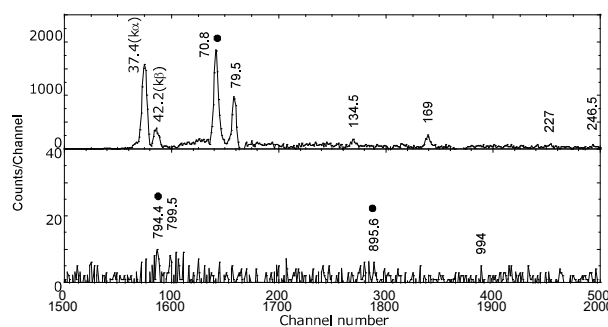
Fig. 1. Coincidence spectrum gated by the 162.4 keV \gamma -ray in the decay of 154 Pr. The closed circles indicate the reported \gamma -rays [1].
