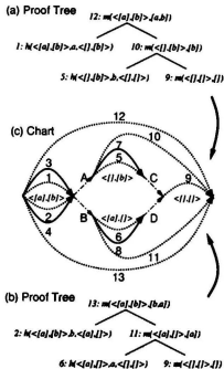
Figure 5.11: Alignment of Indices
