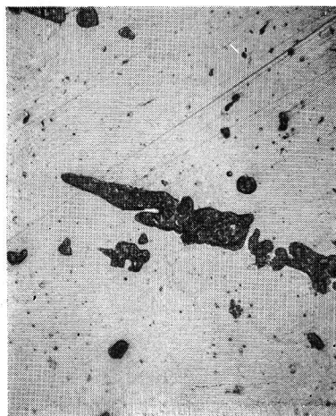
Photo. 2 \times 300 C=0.14%, As=8.31% 800°C. \times 30 min. W.Q. 5% Picral etch. Ferrite + Martensite.
