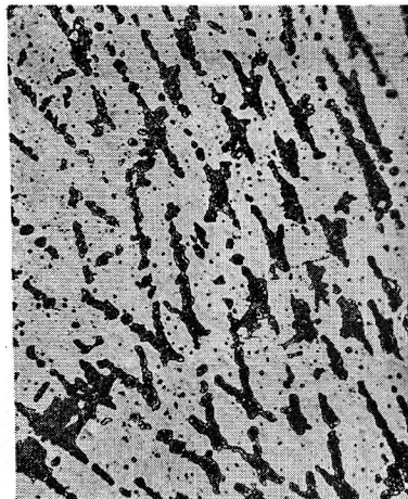
Photo. 4 \times 100 C=0.20%, As=6.43% 880°C. \times 30 min. W.Q. 5% Picral etch. Ferrite + Martensite. (Pearlite partly remains.)
