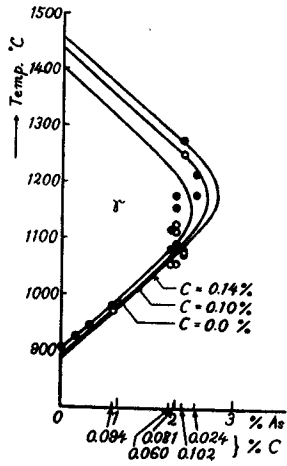
Fig. 5. Shapes of \gamma -loops.
