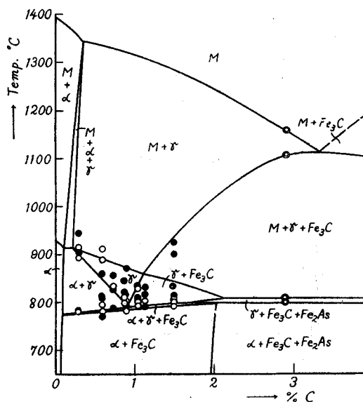
Fig. 13. Section VIII (As≈8.5%).
