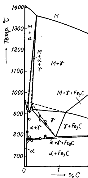
Fig. 12. Section VII (As≈7.5%).
