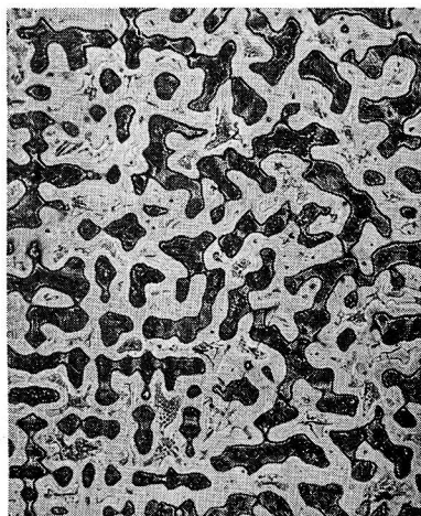
Photo. 13 \times 100 C=0.50%, As=10.05% Cast structure, 5% Picral etch. Austenite Dendrite + ( \gamma -Fe + \text{Fe}_2\text{As} ) Eutectic+Ternary Eutectic+Pearlite in Ferrite Grain.
