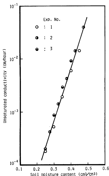
Fig. 10. Relationship between unsaturated conductivity and soil moisture content at 10 cm depth from surface.
