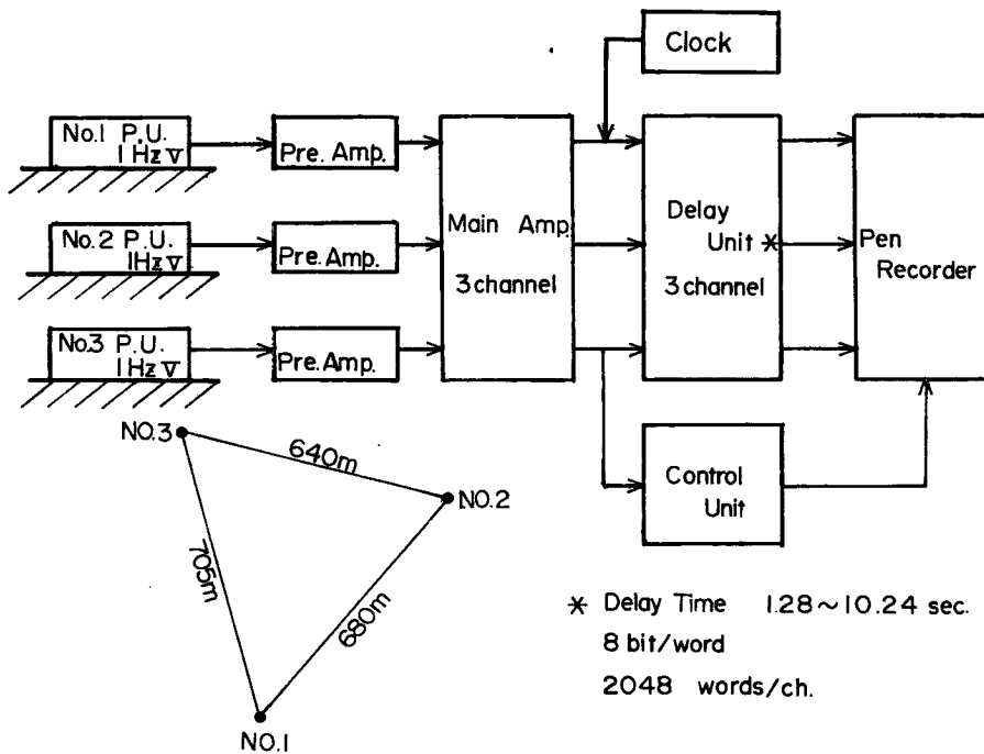
Fig. 5. Block diagram of observing system and ripartite net used.
