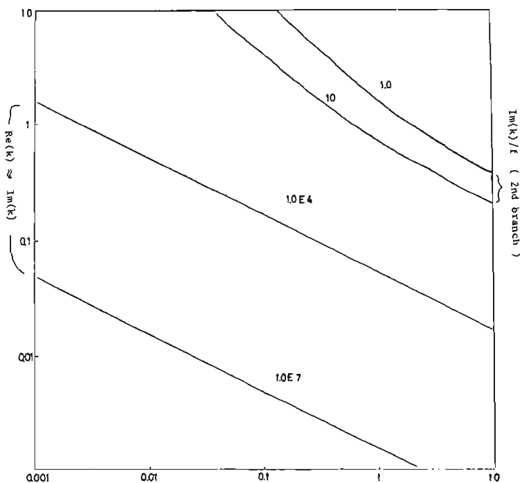
Fig. 5(2). Relation between f and Im(k)/f -second branch of solutions, under \eta=25 and C varied. For higher values of C ( 10^4 and 10^7 ), Re(k)/f is nearly equal to Im(k)/f .
