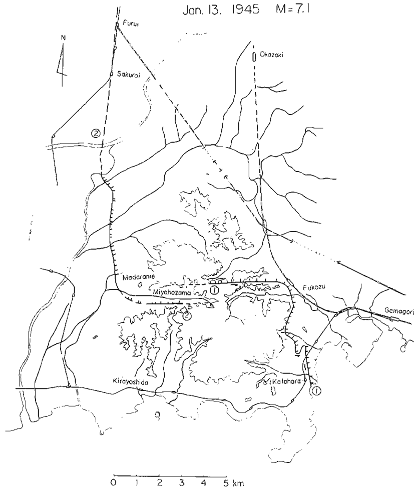
Fig. 11. Faults in the Mikawa earthquake; ①; Fukoju fault, and ②; Yokosuka fault.
