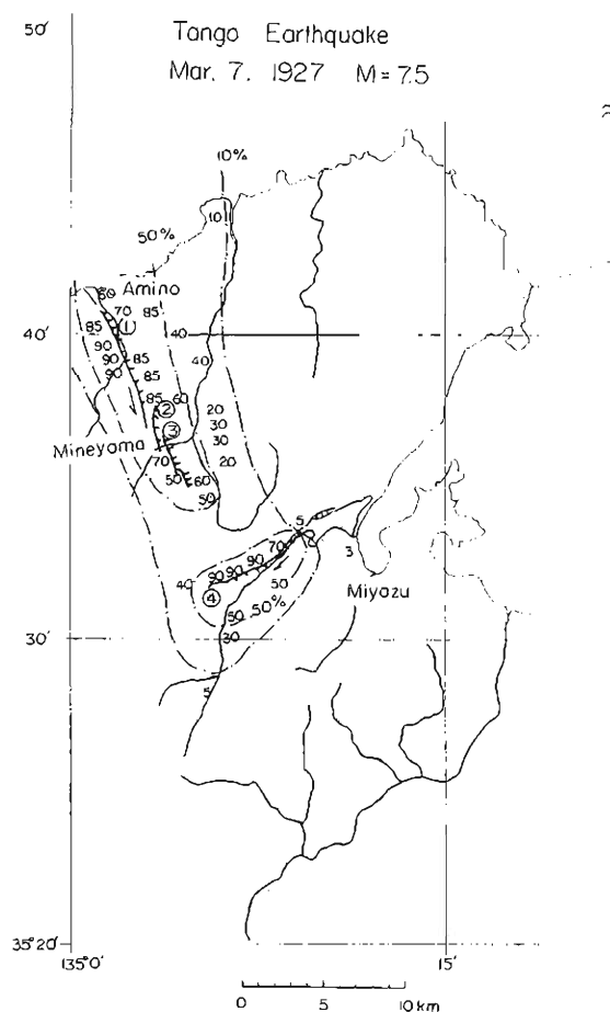
Fig. 8. Faults and percentages of totally collapsed houses in the Tango earthquake; ①; Takahashi fault, ②; Nimbari fault, ③; Nagaoka fault, above three together named the Gomura fault, and ④; Yamada fault.
