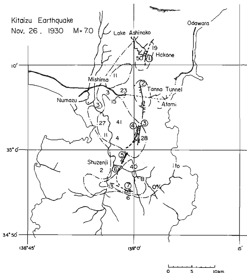
Fig. 9. Faults and percentages of totally collapsed houses in the Kitaizu earthquake; ①; Hakonemachi fault, ②; Tanna fault, ③; Ukihashi-Central fault, ④; Ukihashi-West fault, ⑤; Ōno fault, ⑥; Kadono fault, and ⑦; Himenoyu fault.
