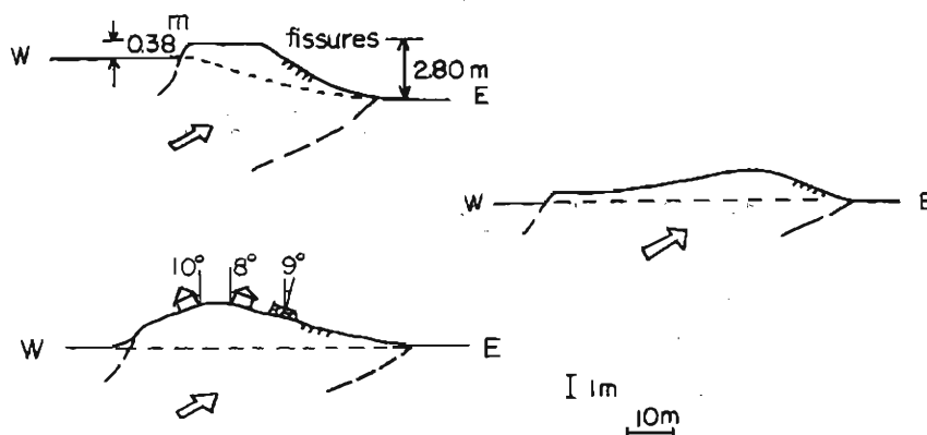
Fig. 16. Mole tracks along the Fukôzu fault in the Mikawa earthquake. (illustrated after Inouye)
