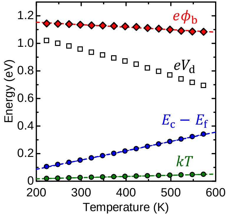
Figure A.4: The temperature dependence of the barrier height in the GaN SBD obtained from the C – V measurements. The values of eV_d , E_c - E_f and kT are also shown. The barrier height almost linearly decreased with elevating temperature.
