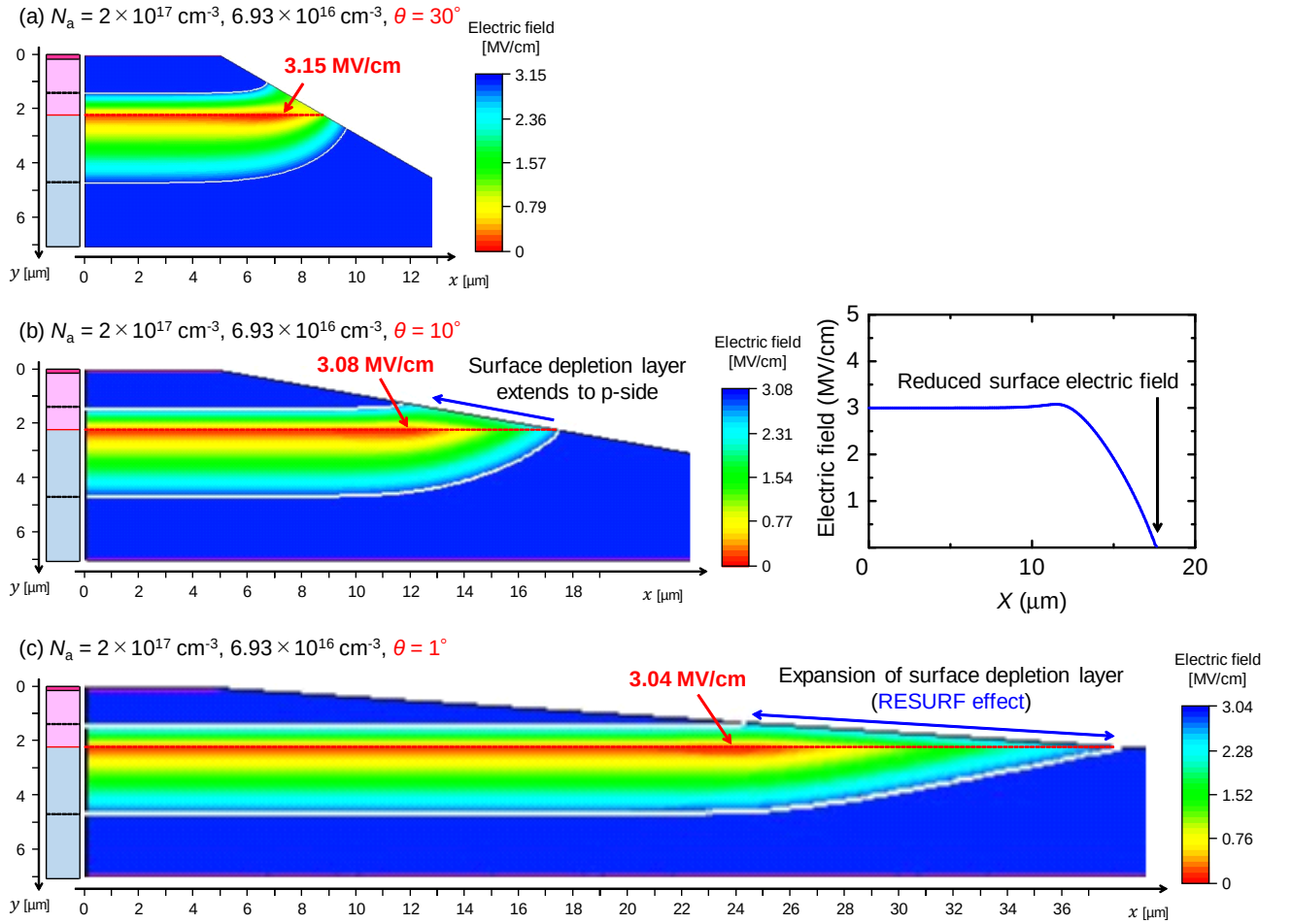
Figure 2.10: Simulated 2-D electric field distributions of the beveled-mesa structures for acceptor concentrations of 2 \times 10^{17} \text{ cm}^{-3} with mesa angles of (a) 30^\circ , (b) 10^\circ and (c) 1^\circ .
