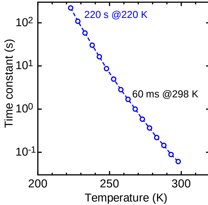
Figure A.13: The temperature dependence of the emission time constant of the E3 trap ( E_C - E_t \sim 0.6 eV). At low temperature, electrons keeps being captured while the C - V measurements, resulting in slight difference of the slope in Fig. A.3.
