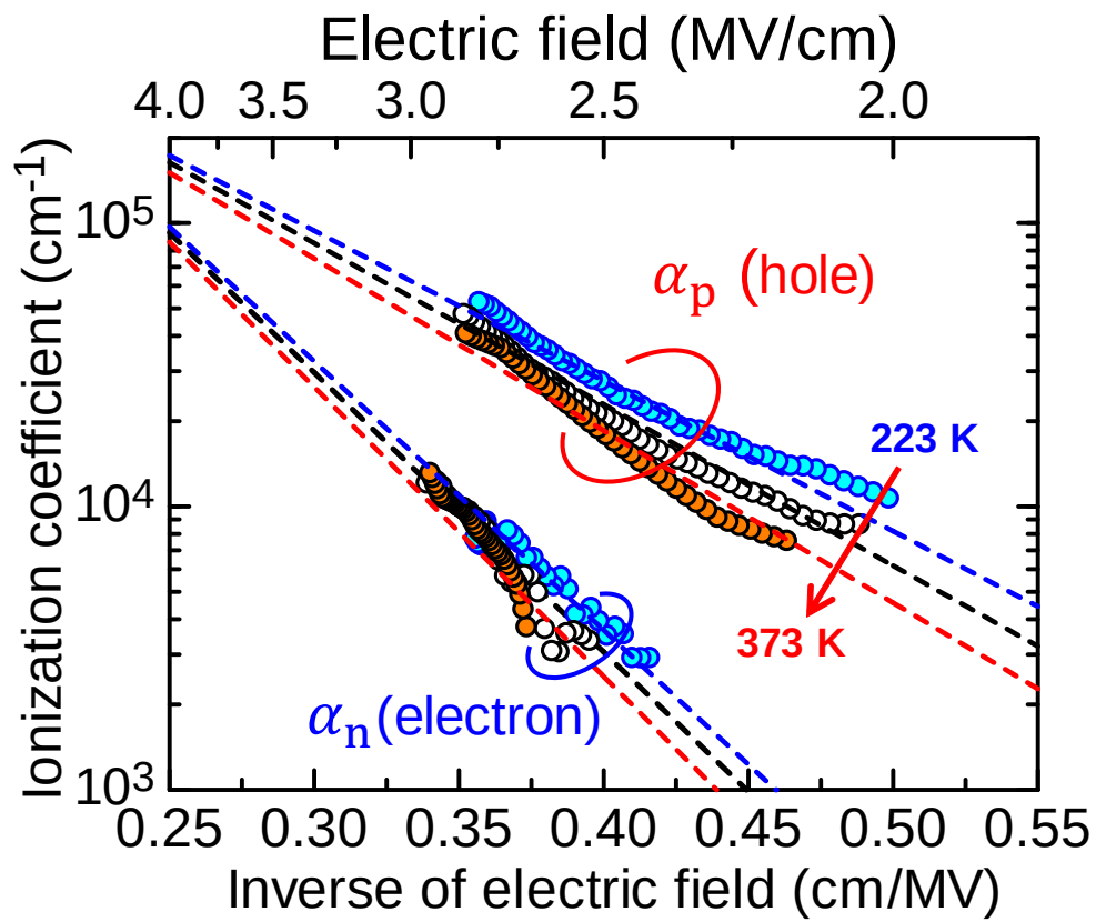
Figure 5.37: Impact ionization coefficients of electrons and holes in GaN obtained at 223, 298 and 373 K. The broken lines indicate the modeled values based on the Okuto-Crowell model [51].
