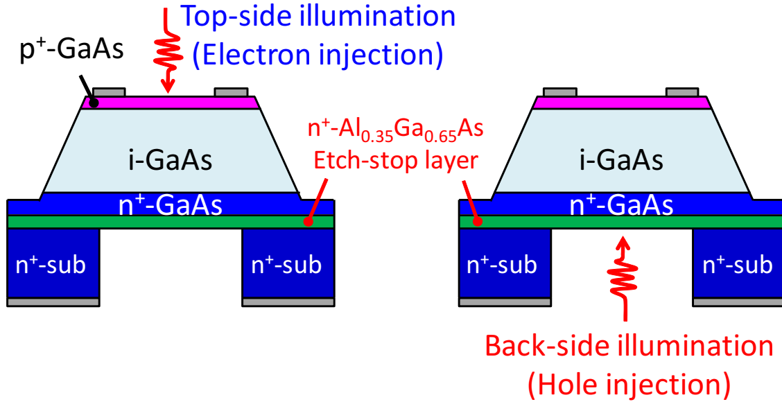
Figure 5.4: Diagrams of the photomultiplication measurement reported by Bulman et al. [10]. For GaAs p - i - n junction diodes with the deep well structure at the back side fomred by selective wet etching utilizing the AlGaAs etch-stop layers, the above-bandgap light ( \lambda = 632.8 nm) was irradiated from the top side and the back side. From the top side and back side illuminations, electron- and hole-injections were obtained, respectively.
