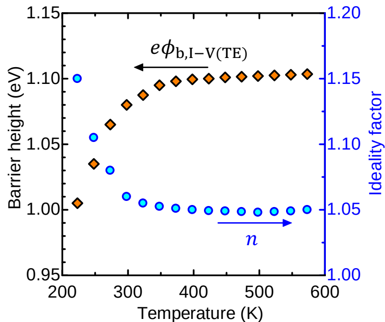
Figure A.6: The temperature dependence of the barrier height obtained by the analysis of the I - V based on the thermionic emission model. The temperature dependence of the ideality factor is also shown.
