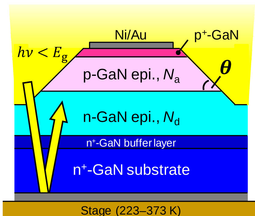
Figure 5.10: Schematic cross section of a GaN p-n junction diode with the double-side-depleted shallow bevel termination. The sub-bandgap light was irradiated to GaN, penetrated into GaN from around the anode electrode, was reflected from the back side electrode and reached p-n junction via multiple reflections. The temperature of the stage was controlled in the range of 223–373 K.
