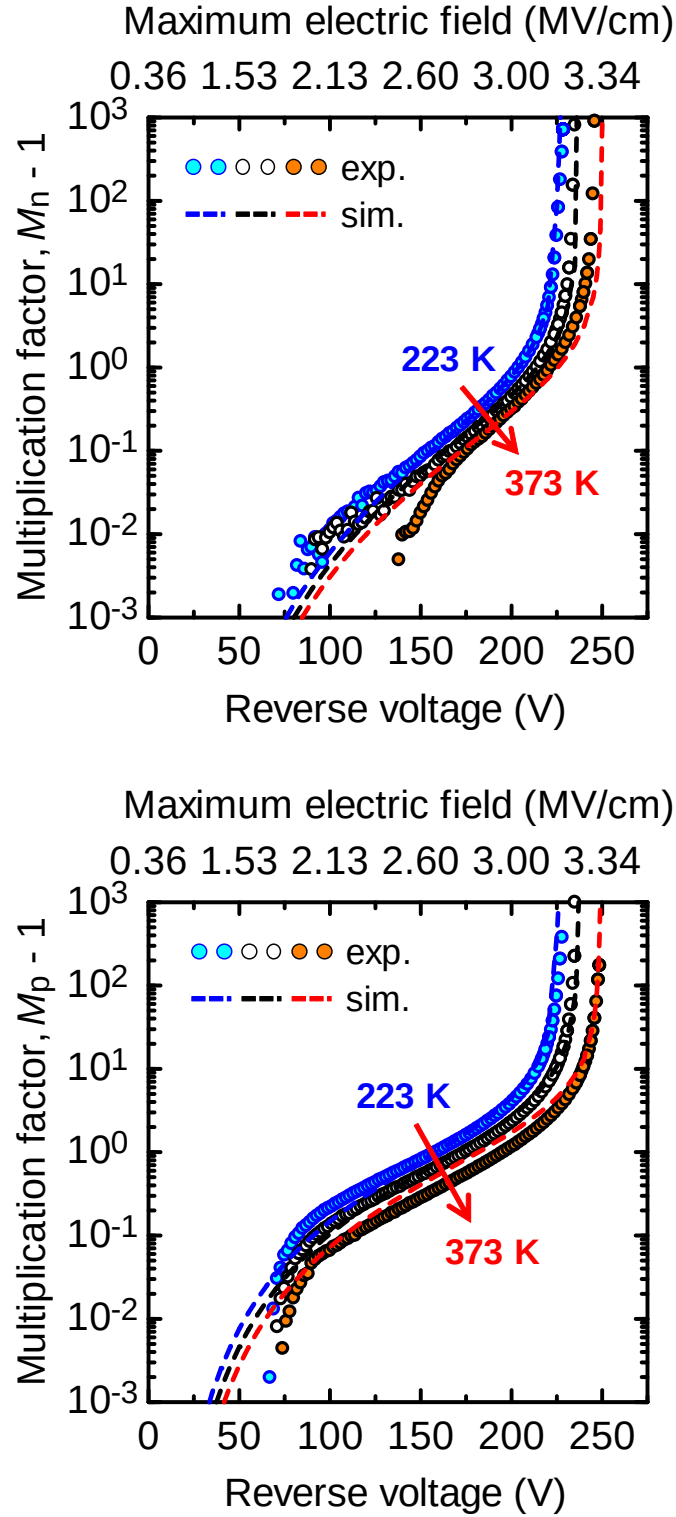
Figure 5.36: Reverse-voltage dependence of the electron- and hole-initiated multiplication factors ( M_n , M_p ) at 223, 298 and 373 K. The simulated curves using the obtained impact ionization coefficients in GaN are also shown as broken lines.
