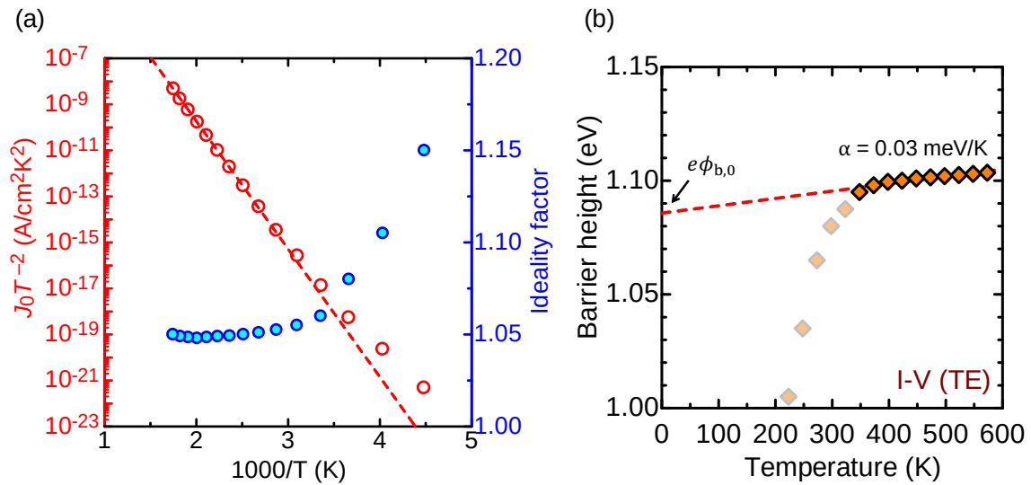
Figure A.14: (a) The Richardson plot of the GaN SBD in this study, and (b) the temperature dependence of the barrier height obtained from the I - V method (based on the TE analysis). The obtained e\phi_{b,0} is indicated.
