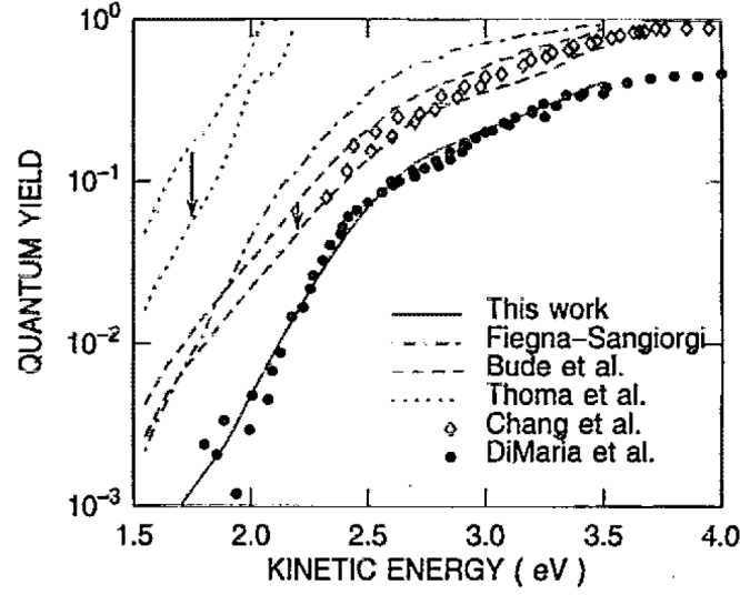
Figure 5.52: The quantum yield for electron-hole pair production as a function of electron kinetic energy in Si reported by Cartier et al. [6]. The threshold energy to cause impact ionization is approximately 1.5E_{g,\text{Si}} .
