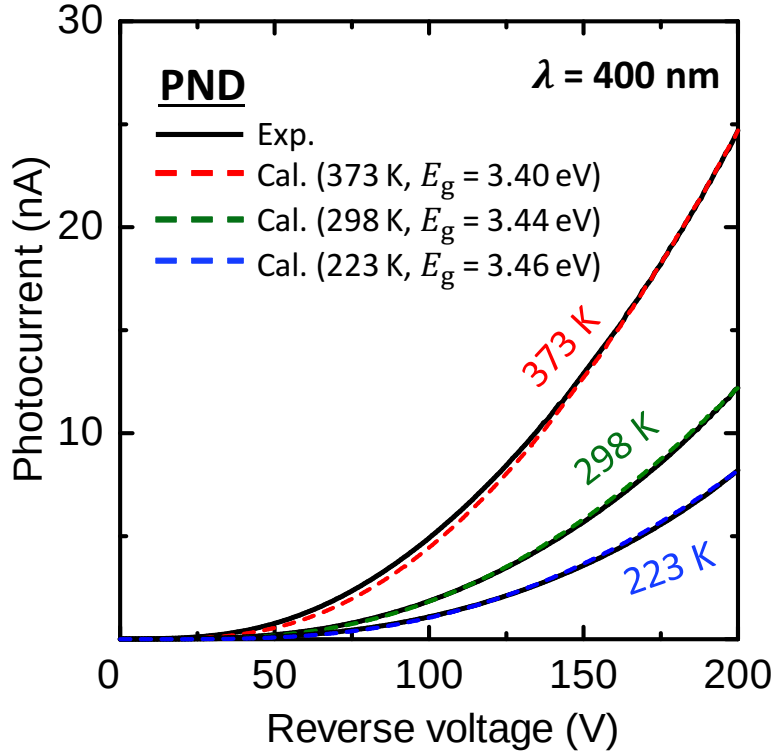
Figure 4.20: Reverse voltage dependence of the photocurrent for 400 nm in the GaN p-n junction diode at 223, 298 and 373 K. With elevating temperature, the photocurrent induced by the FK effect increased, which can be explained by the shrinkage of the bandgap with elevating temperature: the calculated photocurrents with consideration of the temperature dependent bandgap [57] are also shown as broken lines.
