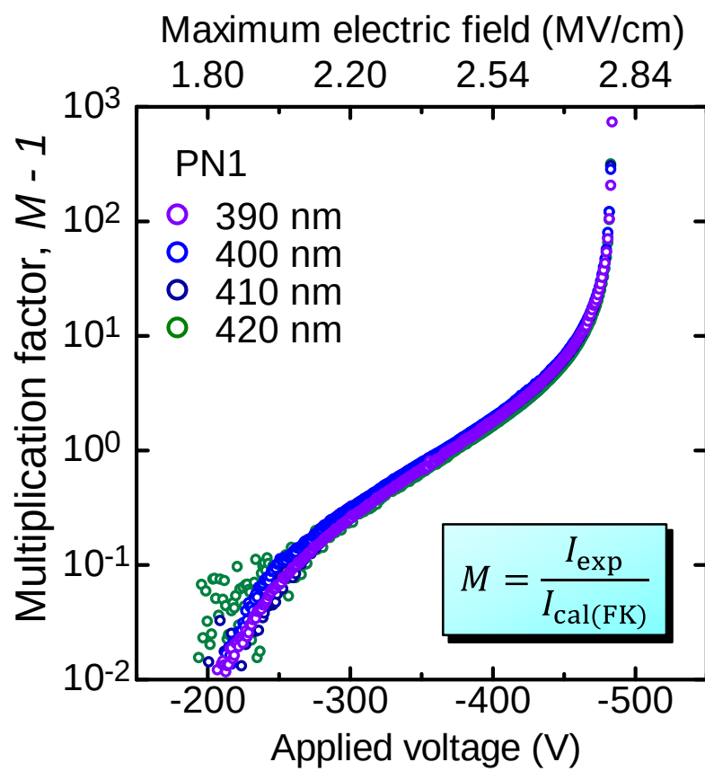
Figure 5.13: Reverse-voltage dependence of the avalanche multiplication factors for 390–420 nm in PN1.
