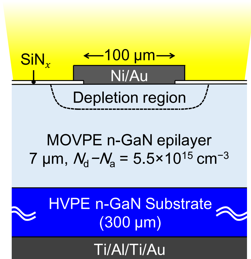
Figure 4.2: Schematic cross section of a Ni/n-GaN Schottky barrier diode used in this study. The wavelength of the incident light was longer than the absorption edge of GaN; therefore, the light penetrated into GaN. The light was reflected by the back-side Ohmic electrode and reached the Ni/GaN interface.
