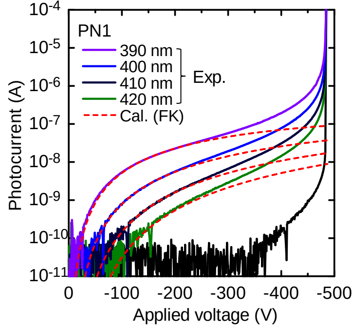
Figure 5.11: Reverse-voltage dependence of the photocurrents for 390–420 nm in the GaN p-n junction diode with the double-side-depleted shallow bevel termination (PN1). The calculated curves of the FK-induced photocurrents are also shown as the red broken lines.
