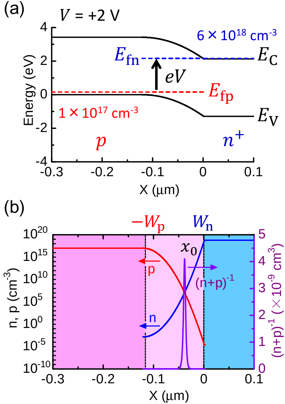
Figure B.5: (a) Band diagram of the p^-/n^+ junction and (b) the distributions of electrons ( n ), holes ( p ) and (n+p)^{-1} under an applied voltage of +2 V. The SRH recombination intensively occurs at the depth x_0 , which is very close to the peak of (n+p)^{-1} .
