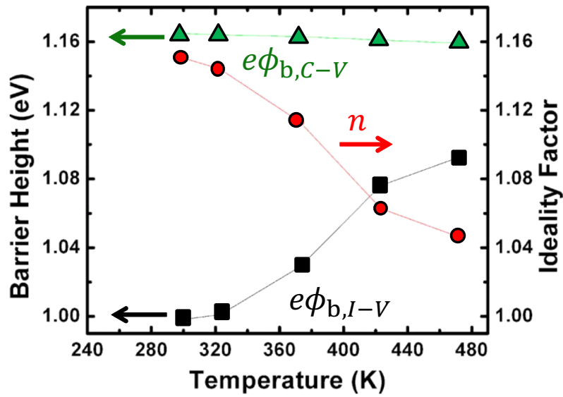
Figure A.1: The temperature dependence of the barrier height obtained by C - V and I - V measurements reported by Zhou et al. [22]. The temperature dependence of the ideality factor is also shown. Due to the non-ideal I - V characteristic, the inconsistent results were obtained.
