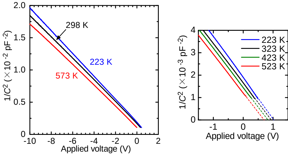
Figure A.3: The capacitance–voltage characteristics of the GaN SBD in the range of 223–573 K. The magnification near zero bias is also shown. The plots shifted to the negative side with elevating temperature, indicating the decrease in the built-in potential.
