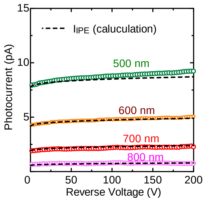
Figure 4.11: Comparison between the experimental photocurrents induced by IPE and the calculated photocurrent considering the effect of the image force lowering.
