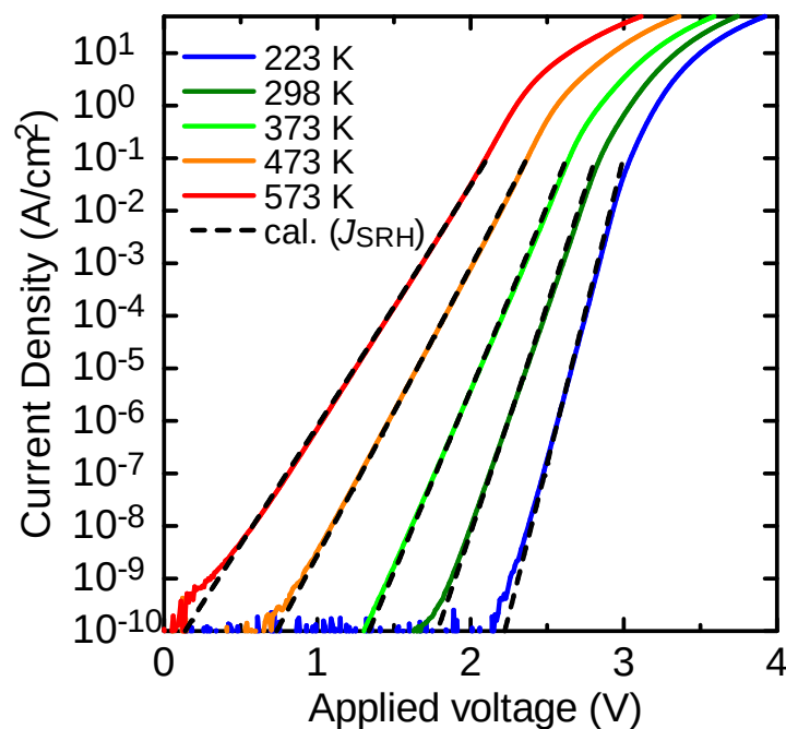
Figure B.7: Forward I - V characteristics in the GaN p-n + junction diode at 223–573 K. The calculated SRH recombination currents at each temperature are also shown as broken lines.
