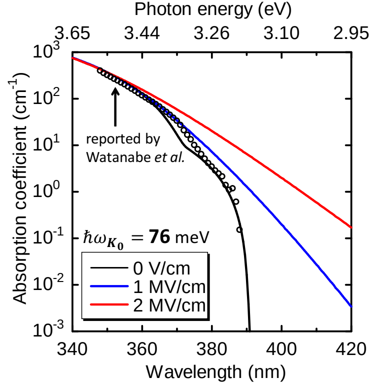
Figure C.5: Wavelength dependence of the calculated absorption coefficient for 4H-SiC under electric fields of 0, 1, and 2 MV/cm. The LA-mode phonon ( \hbar\omega_{K_0} = 76 \text{ meV} ) was considered in the calculation. The calculated absorption coefficient under 0 V/cm (black line) shows good agreement with the reported values (open circles) [42].
