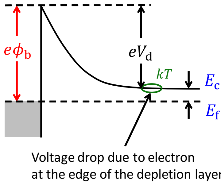
Figure 4.4: Energy diagram at a Schottky junction. A barrier height is a sum of built-in potential, a difference between a conduction band minimum and a fermi level, and a voltage drop at a depletion layer edge.
