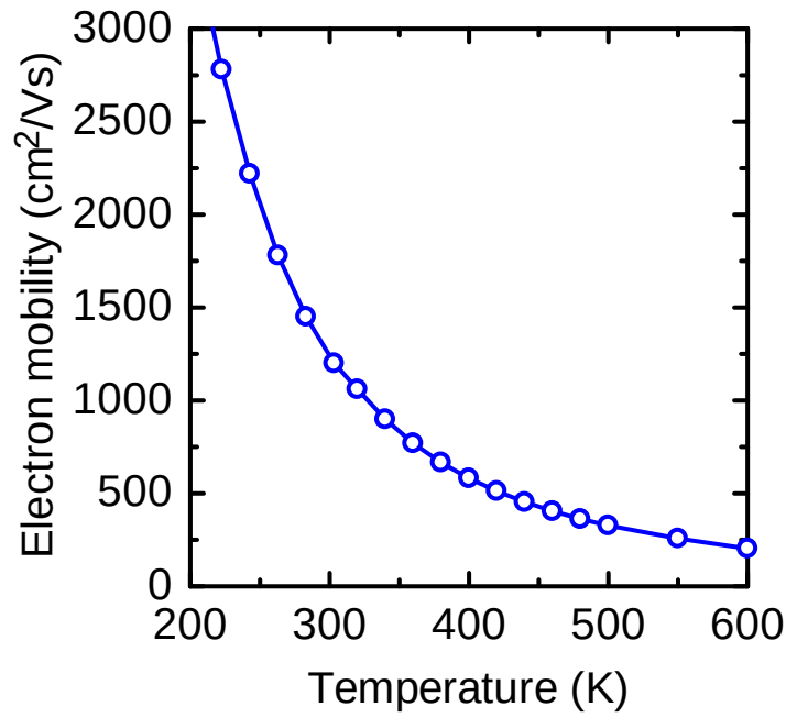
Figure A.8: The temperature dependence of the electron mobility for the carrier concentration of 4 \times 10^{15} \text{ cm}^{-3} measured by Sawada et al. [26].
