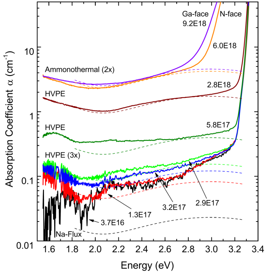
Figure 4.22: Sub-bandgap optical absorption coefficient for bulk GaN samples at room temperature reported by Pimputkar et al. [52]. Dashed lines represent calculated values for phonon-assisted free carrier absorption.
