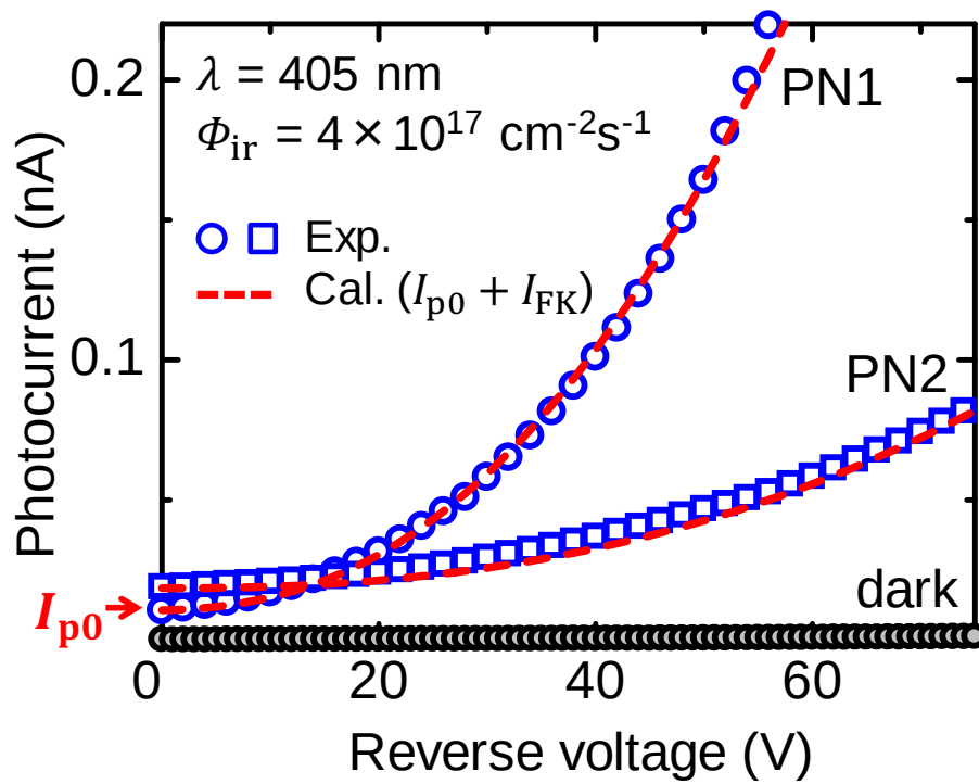
Figure C.9: Reverse current-voltage characteristics in the 4H-SiC(11 \bar{2} 0) PNDs (PN1 and PN2) under illumination with sub-bandgap light ( \lambda = 405 nm) at 298 K. The curve calculated taking into consideration the FK effect ( I_{p0} + I_{FK} ) is also shown as the red dashed line.
