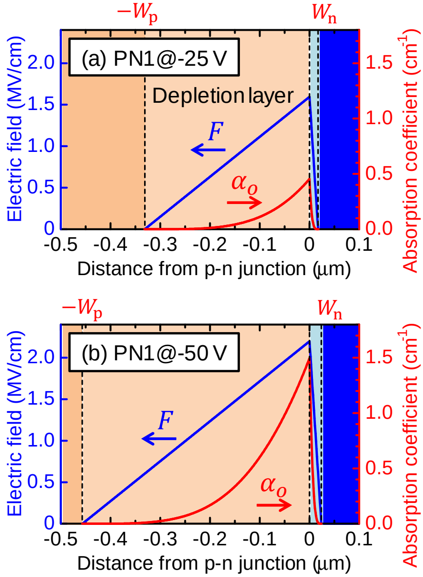
Figure C.12: Distributions of electric field and the absorption coefficient for \lambda = 405 \text{ nm} in PN1 at the reverse voltage of (a) 25 V and (b) 50 V.
