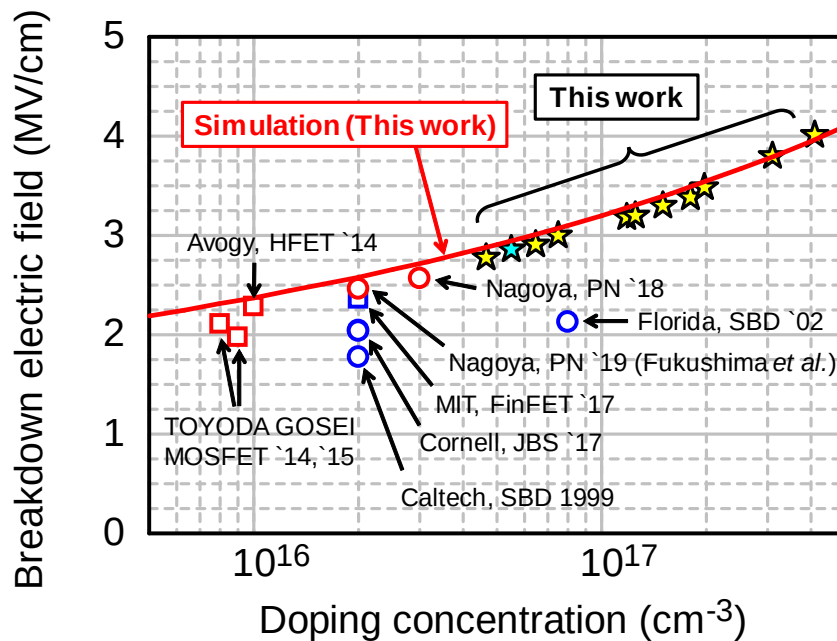
Figure 5.39: Critical electric field versus doping concentration in non-punch-through GaN p-n junctions. The experimental data of the breakdown electric field reported previously [43, 54, 61–66, 68, 70, 71] are also shown.
