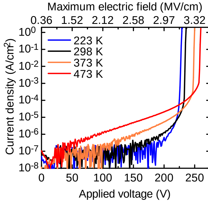
Figure 5.23: Reverse I - V characteristics of the GaN p-n junction diode at 223, 298, 373 and 473 K. The breakdown voltage increased almost linearly with elevated temperature.
