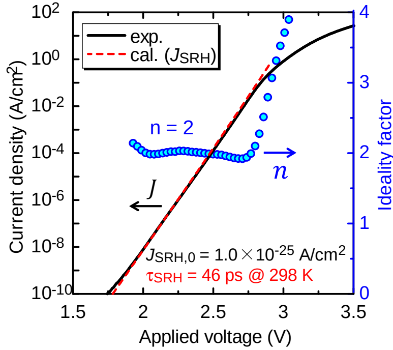
Figure B.3: Forward current-voltage characteristics of the GaN p-n junction diode. The ideality factor as a function of the applied voltage is shown blue circles. The calculated recombination current is shown as red broken line, and the \tau_{\text{SRH}} = 46 ps in homoepitaxial p-GaN was obtained.
