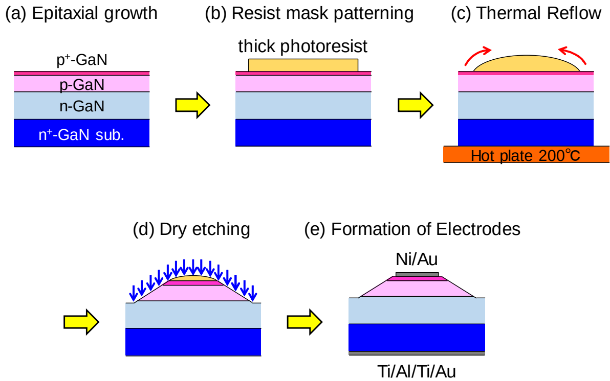
Figure 2.12: Fabrication process flow of a GaN p-n junction diode with beveled-mesa termination.
