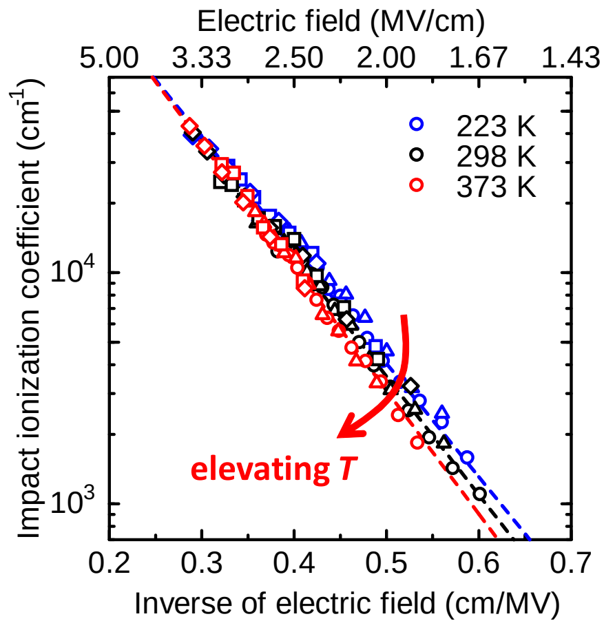
Figure 5.19: The effective impact ionization coefficient ( \alpha ) versus the inverse of the electric field at 223, 298 and 373 K.
