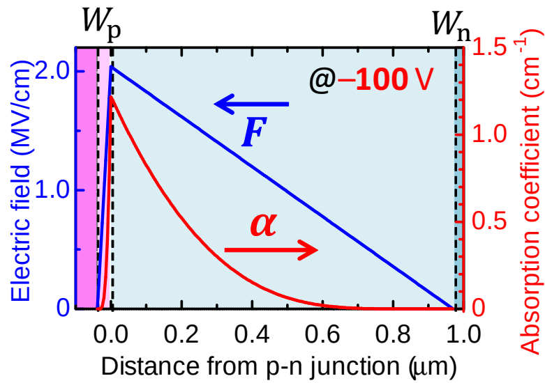
Figure C.6: The distribution of the electric field and the absorption coefficient for 405 nm in the 4H-SiC PND under the reverse bias of -100 \text{ V} .
