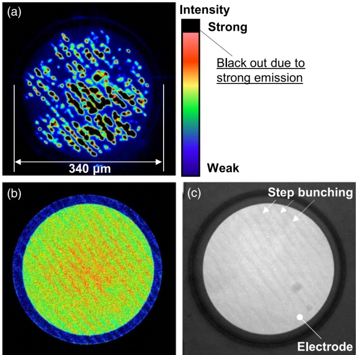
Figure 3.17: (a) Emission microscopy image of the p-n junction diode with high reverse bias of -879\text{ V} applied. (b) Emission microscopy image with forward bias of 2.5\text{ V} applied. (c) Optical microscopy image. These results are reported in [49].
