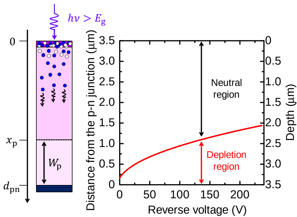
Figure 5.26: Extention of the depletion layer as a function of the reverse bias voltage. x_p determines the voltage dependence of the electron diffusion current.
