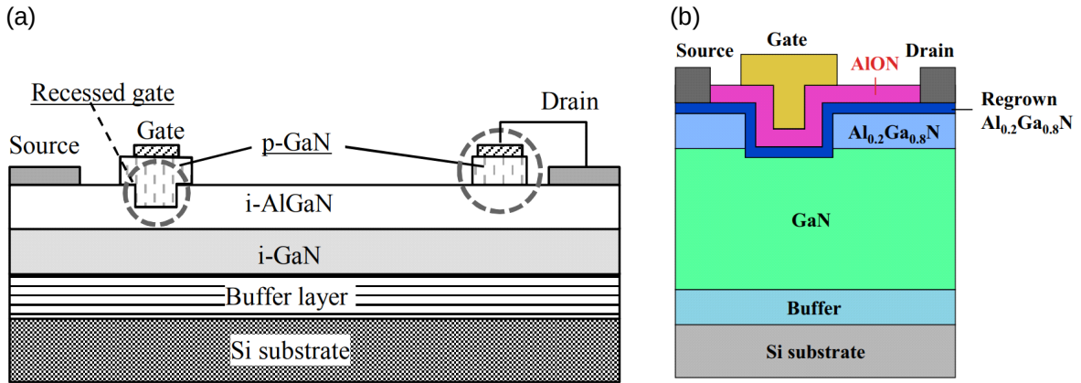
Figure 1.8: Device structures of (a) the hybrid-drain-embedded GaN GIT [78] fabricated on a Si substrate and (b) the AlGaN/GaN MIS-HFET using AlON gate insulator fabricated on a Si substrate [79]
