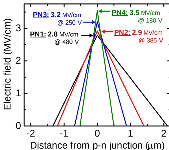
Figure 3.11: The calculated electric field distributions for the parallel-plane junctions of PN1–PN4 at the breakdowns. The breakdown electric fields of approximately 2.8, 2.9, 3.2 and 3.5 MV/cm were obtained.
