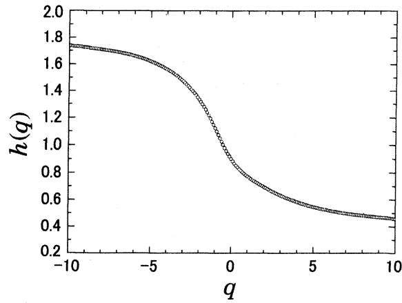
Fig. 6: The generalized Hurst exponent h(q) for the moment q .
