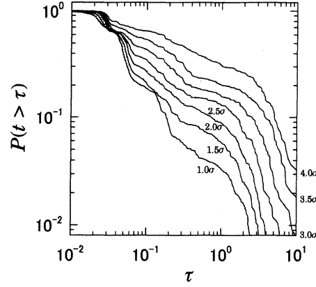
Fig. 4: Return interval distribution for the various values of threshold, \sigma < q < 4.5\sigma , where \sigma denotes the standard deviation of magnetic fluctuations. We can observe that the return interval distribution is closer to a straight line with the slope of the log-log plot when the threshold value is larger than 4\sigma .
