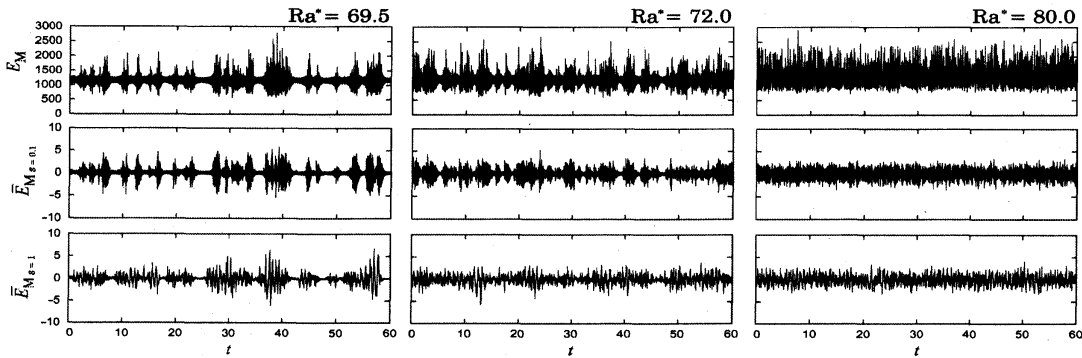
Fig. 1: A part of time-series data of intermittent magnetic fluctuations near the critical Hopf bifurcation point on different timescales s ( s=0.1 , s=1.0 ) for (a) r=69.5 , (b) r=72 and (c) r=80 , respectively (from left to right).
