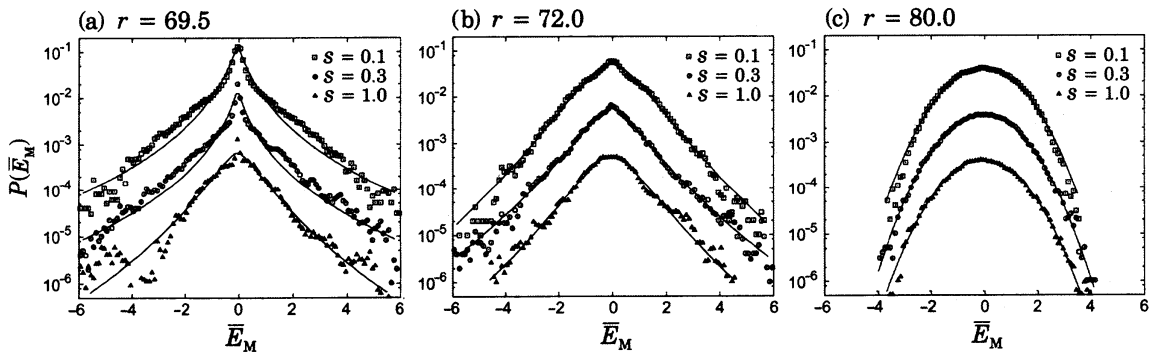
Fig. 2: Standardized probability density functions (PDF) of magnetic fluctuations on different timescales s approximated by Lognormal distribution for (a) r=69.5 , (b) r=72 and (c) r=80 , respectively (from left to right). The PDFs on scales s=0.1(\square) , s=0.3(\text{circle}) and s=1.0(\Delta) , respectively (from top to bottom). The PDFs for r = 80 show almost a Gaussian.
