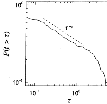
Fig. 5: Return interval distribution of extreme events for the larger threshold value 4\sigma , where \sigma denotes the standard deviation of magnetic fluctuations. We can clearly observe the tail exponent.
