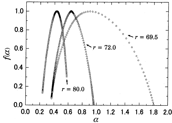
Fig. 7: Singularity spectrum for intermittent chaos of magnetic fluctuations.
