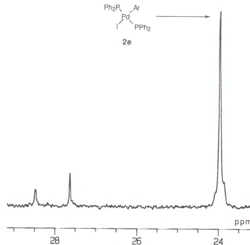
Figure 12. ^{31}\text{P}\{^1\text{H}\} NMR (109 MHz) spectrum of the reaction mixture (at ca. 75% conversion) of the coupling of tributyl(phenylethynyl)tin with \text{Ar-I} catalyzed by \text{Ph}_3\text{P-Pd}_2(\text{dba})_3 ( \text{Ph}_3\text{P}/\text{Pd} = 2 ) in THF at 50 °C.
