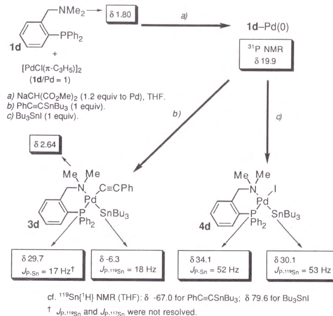
Figure 5. ^{31}\text{P}\{^1\text{H}\} , ^{119}\text{Sn}\{^1\text{H}\} and ^1\text{H} NMR (THF- d_8 ) parameters (chemical shift and J_{\text{Sn-P}} ) of Pd(0)/ 1d and its reaction products with \text{PhC}\equiv\text{CSnBu}_3 or \text{Bu}_3\text{SnI} .
