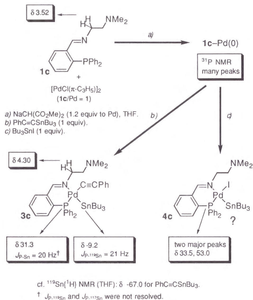
Figure 4. ^{31}\text{P}\{^1\text{H}\} , ^{119}\text{Sn}\{^1\text{H}\} and ^1\text{H} NMR (THF- d_8 ) parameters (chemical shift and J_{\text{Sn-P}} ) of Pd(0)/ 1c and its reaction products with \text{PhC}\equiv\text{CSnBu}_3 or \text{Bu}_3\text{SnI} .
