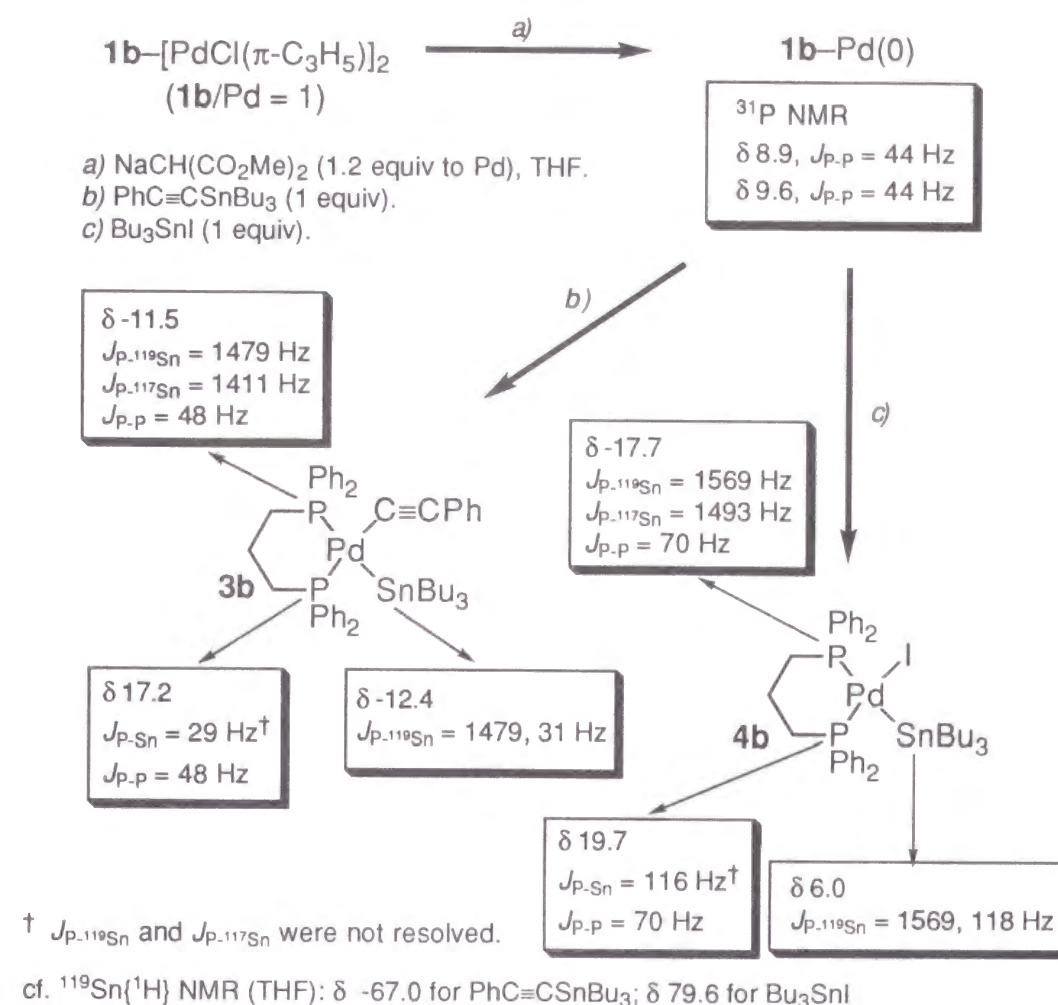
Figure 3. ^{31}\text{P}\{^1\text{H}\} and ^{119}\text{Sn}\{^1\text{H}\} NMR (THF) parameters (chemical shift, J_{\text{Sn-P}} and J_{\text{P-P}} ) of Pd(0)/ 1b and its reaction products with \text{PhC}\equiv\text{CSnBu}_3 or \text{Bu}_3\text{SnI} .
