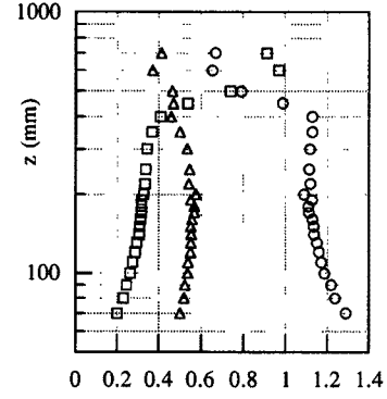
Fig. 3 Profiles of the components of turbulent kinetic energy: \circ , u'^2/k ; \triangle , v'^2/k ; \square , w'^2/k .
