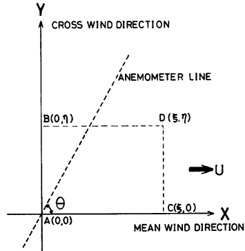
Fig. 2. Co-ordinate used in order to obtain horizontal space correlations.
