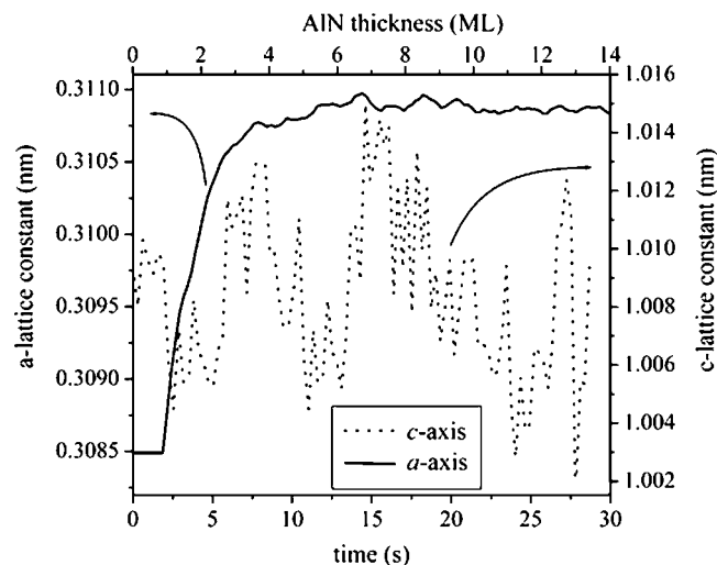
FIG. 3. Lattice relaxation process for AlN on 4H-SiC (1-100) determined from variations of [11-20] and [0001] RHEED streak spacings with AlN growth time. 4H-SiC reference values ( 950^\circ\text{C} ) taken as a = 0.3085 nm, c = 1.0094 nm.
