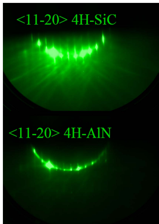
FIG. 2. (Color online) RHEED patterns ( [11-20] azimuth) from 4H-SiC substrate (top) and after growth of 250 nm AlN (bottom).
