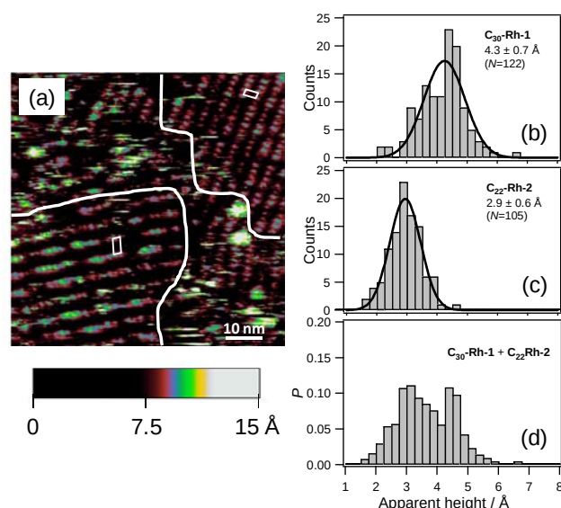
Fig. 4 (a) An STM image of a 10:1 mixed solution of C 22 -Rh-2 ( 1.5 \times 10^{-6} M) and C 30 -Rh-1 ( 1.5 \times 10^{-7} M) ( 75 \times 75 nm 2 , I_{\text{set}} = 30 pA, V_{\text{bias}} = -1.0 V) at the 1-octanoic acid-HOPG interface in the constant current mode. Histograms of apparent height in the domain of (b) C 30 -Rh-1 , (c) C 22 -Rh-2 , and (d) both C 30 -Rh-1 and C 22 -Rh-2 . The contribution in counts from each domain was normalized to 1:1 in histogram (d).
