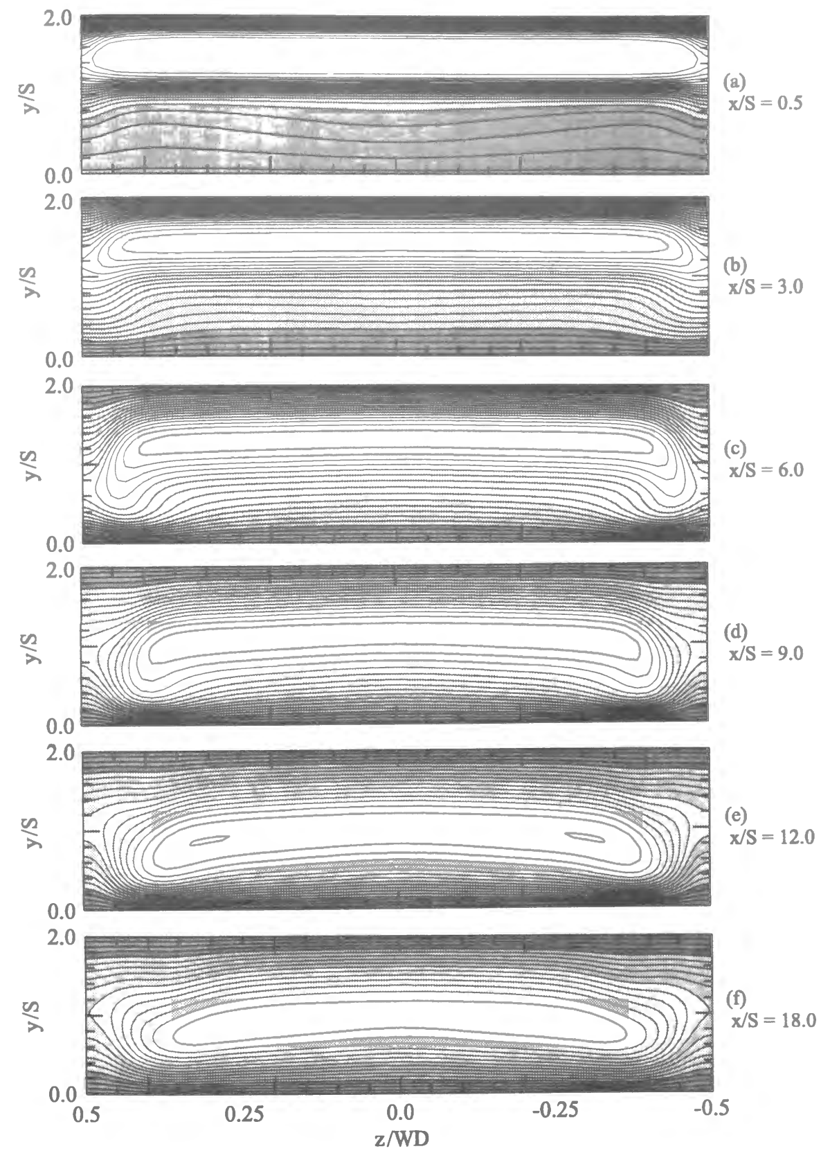
Figure 3.10: Temperature contour ( AR=8 ).
