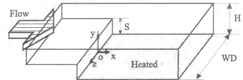
Figure 7.1: Computational domain.
