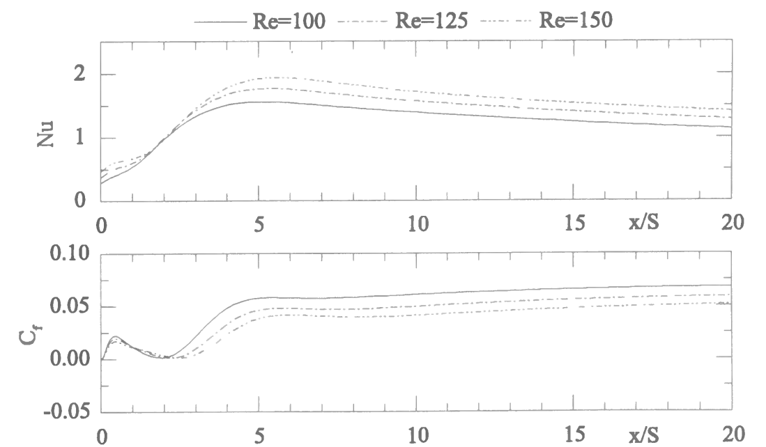
Figure 4.16: Effect of Re at the same Ri^* .
