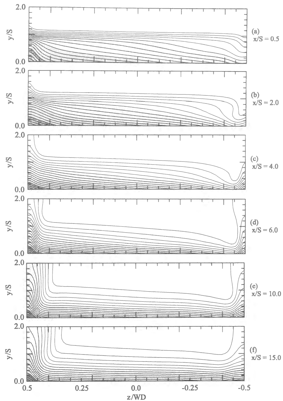
Figure 5.22: Temperature contours.
