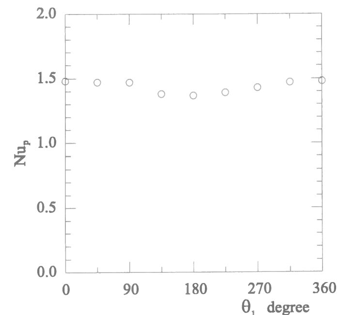
Figure 5.7: Effect of \theta_1 on the peak Nu along the centerline(3-D).
