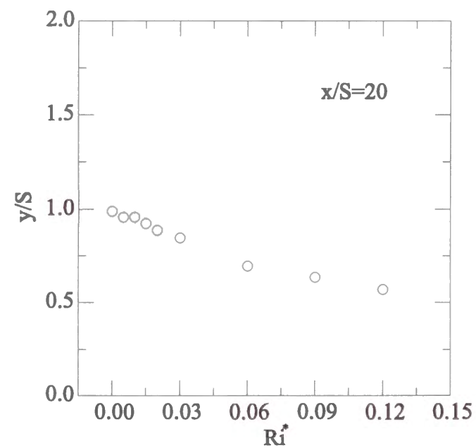
Figure 4.6: y -position of maximum U .
