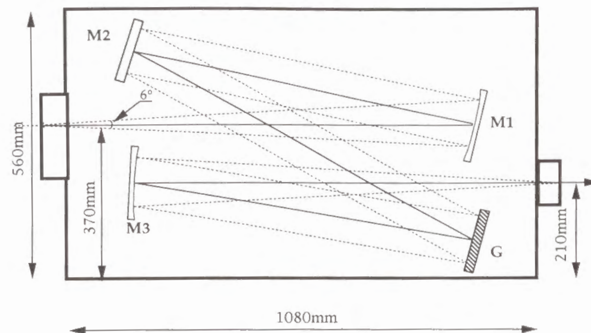
M1: concave mirror, M2: flat mirror G : grating, M3: concave mirror
