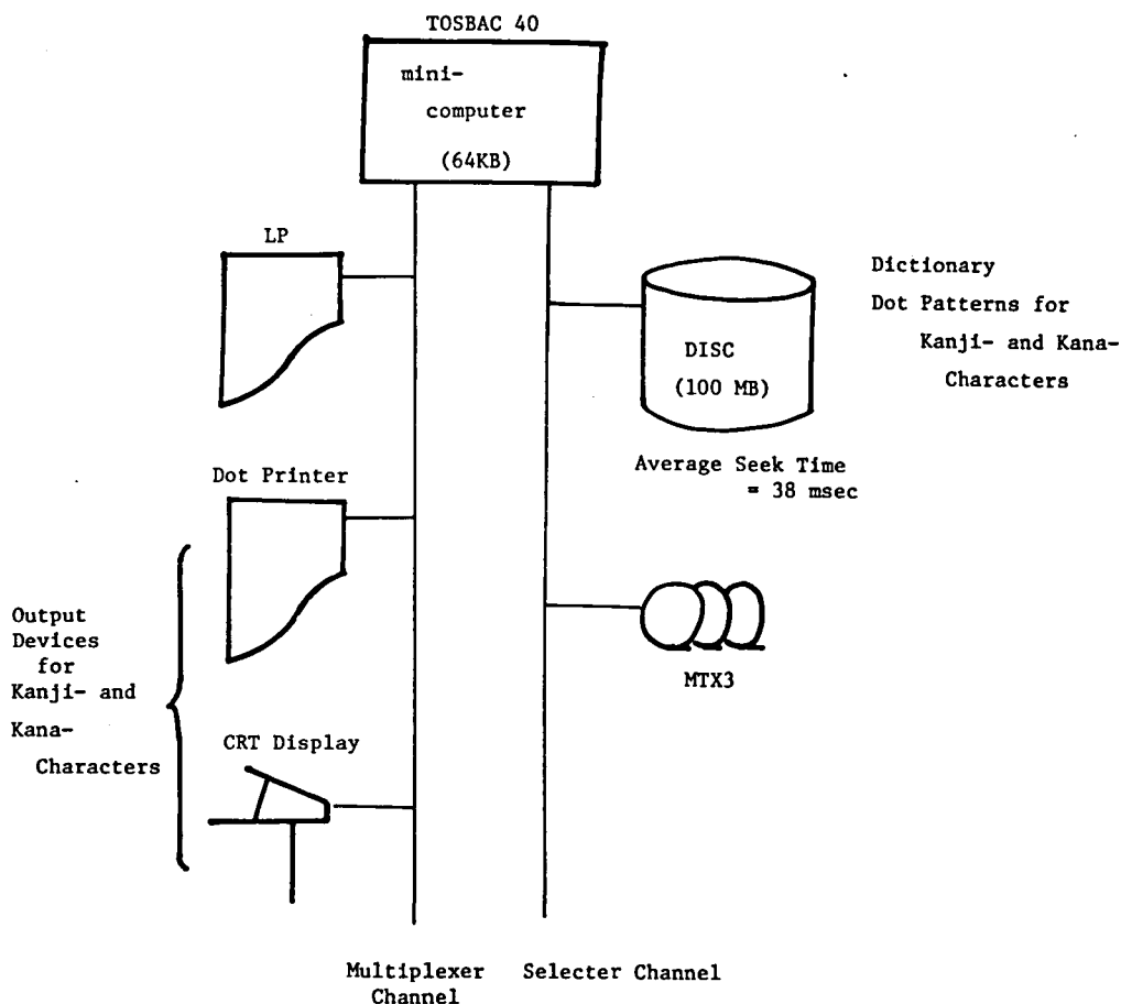
Fig. VI-14 Computer System
