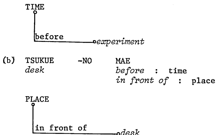
Fig. III-10 Results of Analysis of Noun and Prepositional Noun Phrase
