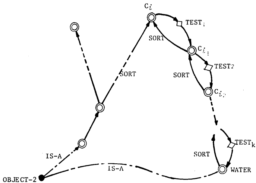
Fig. V-24 Step 5 ( C_i is the common super concept of C_0 and WATER)
