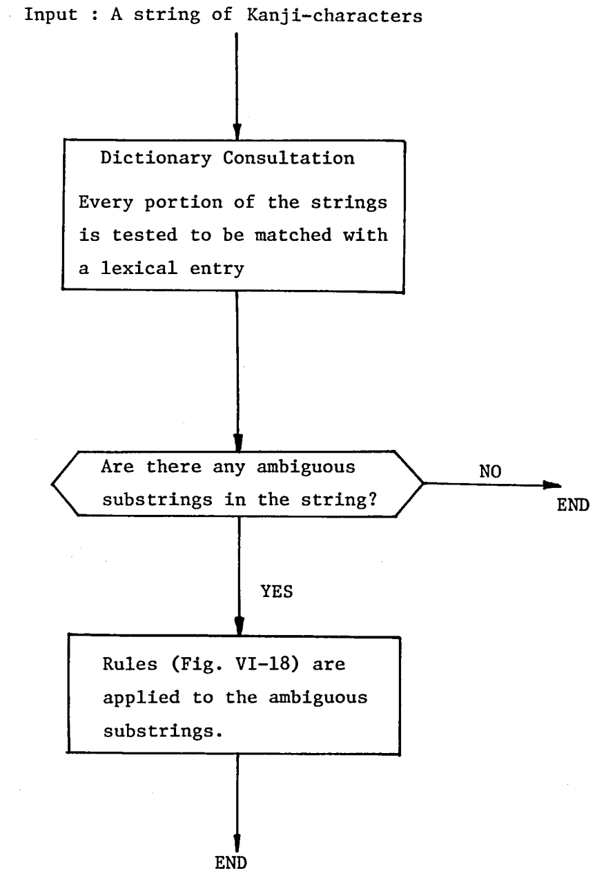
Fig. VI Flow Chart of the Procedure
