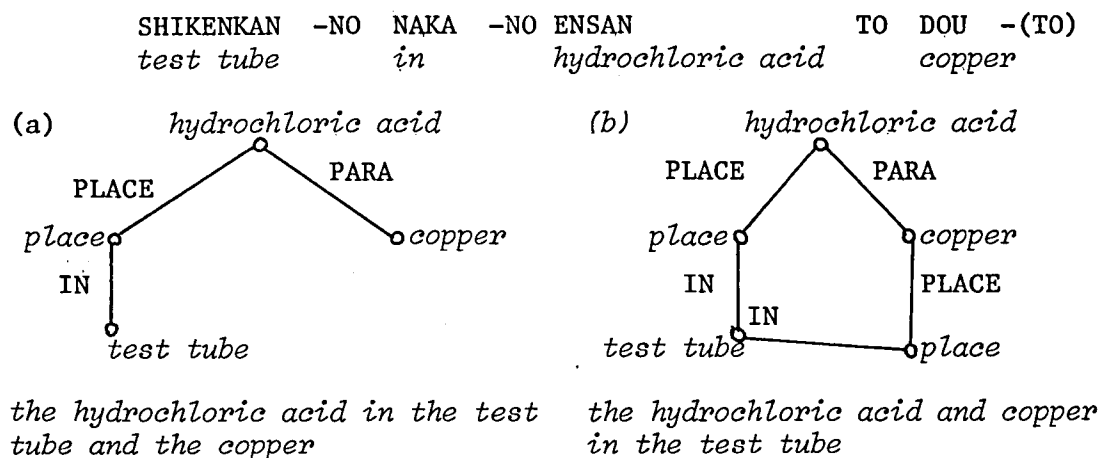
Fig. III-14 Two Different Constructions According to the Two Different Determinations of the Left End of the Conjoined Phrase
