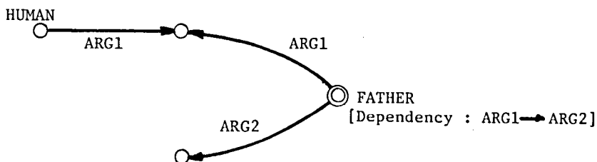
Fig. V-7 Representation of the Fact (\forall x)(\text{HUMAN}(x) \longrightarrow \text{FATHER}(x, f(x)))
