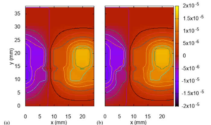
Fig. 9. Snapshots of the vector potential distribution and magnetic flux lines given by (a) motor MOR and (b) FE EC analysis.
