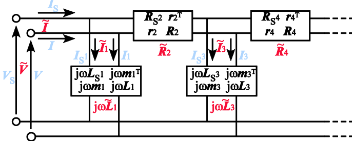
Fig. 4. Matrix Cauer form for the stator domain corresponding to Fig 3(a).
