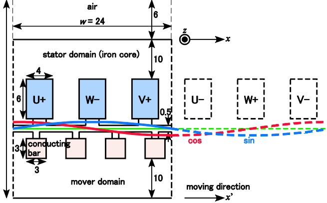
Fig. 2. Linear induction motor (unit: millimeter).
