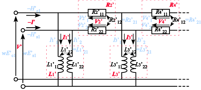
Fig. 5. Matrix Cauer form corresponding to Fig. 3(c) when I' = [H'_{c1}, H'_{s1}] .
