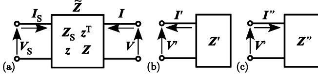
Fig. 3. Multiport transfer functions: (a) stator domain, (b) mover domain to be connected with stator domain, and (c) mover domain generated by the CLN.
