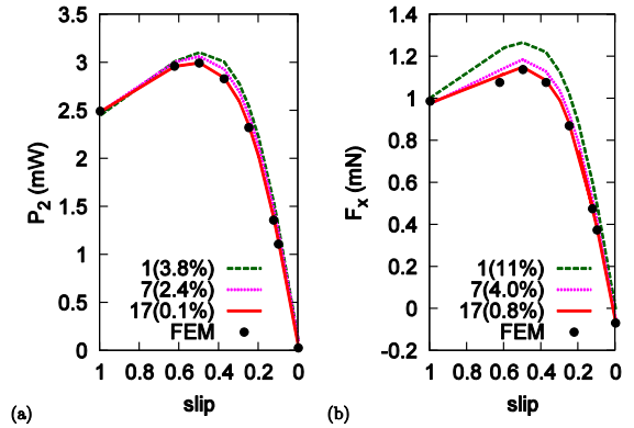
Fig. 8. Speed dependence of (a) the air-gap power and (b) the thrust force. Discrepancies from FE EC analysis at s = 0.5 are indicated in parentheses.
