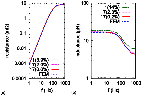
Fig. 7. Frequency dependence of the input impedance: (a) resistive and (b) inductive components. Discrepancies at 100 Hz are shown in parentheses.
