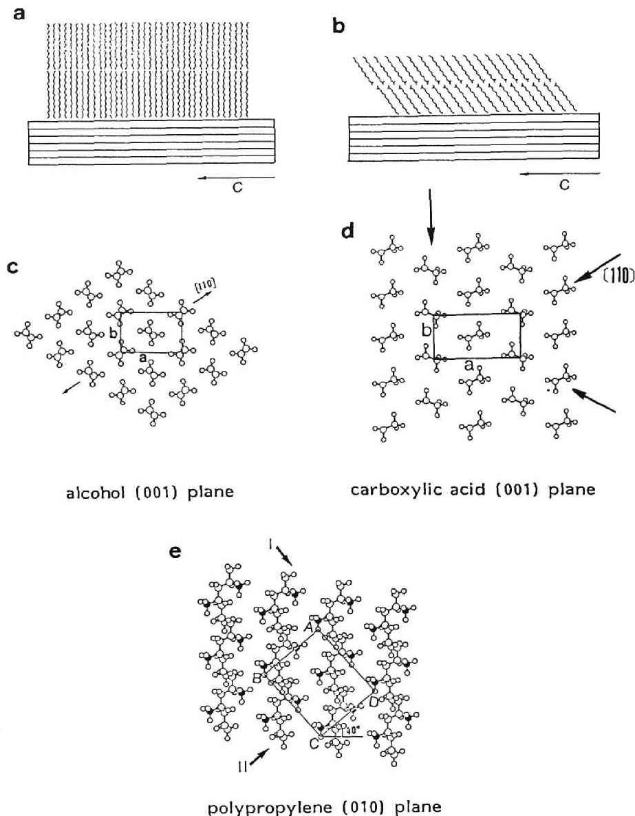
Fig. 4-9 (a) illustration of flat-on lamellar crystal of n-alcohol with -form, (b) illustration of flat-on lamellar crystal of n-carboxylic acid, (c) molecular arrangement of (001) plane of n-alcohol crystal with \beta -form, (d) end methyl group arrangement of carboxylic acid crystal with C'-form and (e) molecular arrangement of polypropylene (010) surface. In (c), (d) and (e) large and small circles mean carbon atoms and hydrogen atoms, respectively. In (e), there is a rectangle ABCD which is a two-dimensional lattice of iPP (010) plane. The spacings of this lattice are as follows; AB=0.846nm and AD=1.005nm.
