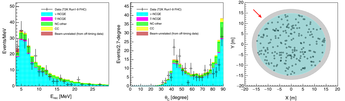
FIG. 7. Distributions of E_{\text{rec}} (left), \theta_C (middle), and vertex (right) from the FHC sample. In the right panel, the red arrow indicates the beam direction and the gray and sky blue regions correspond to the ID and FV, respectively.
