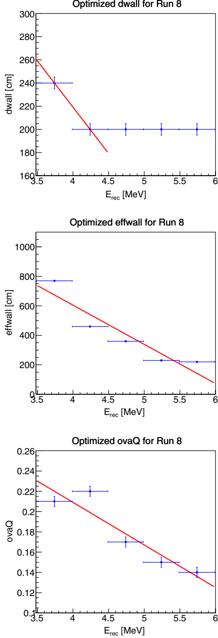
FIG. 3. Optimized cut values for dwall (top), effwall (middle), and ovaQ (bottom), in each low energy bin for one of the FHC mode runs (Run 8). Vertical bars on each point represent the bin width used in parameter scans. Red lines represent linear fits to the distributions and are used for the cut values. Events with parameter values above the lines are used in the analysis. The fit regions for dwall and effwall are explained in the text.
