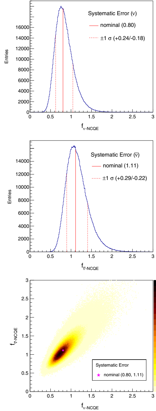
FIG. 11. Results of the pseudoexperiments on the scale factors when the numbers of events are varied based on the systematic uncertainties: f_{\nu\text{-NCQE}} = 0.80^{+0.24}_{-0.18} and f_{\bar{\nu}\text{-NCQE}} = 1.11^{+0.29}_{-0.22} . The dominant uncertainty source is the secondary- \gamma production model as described in the text.
