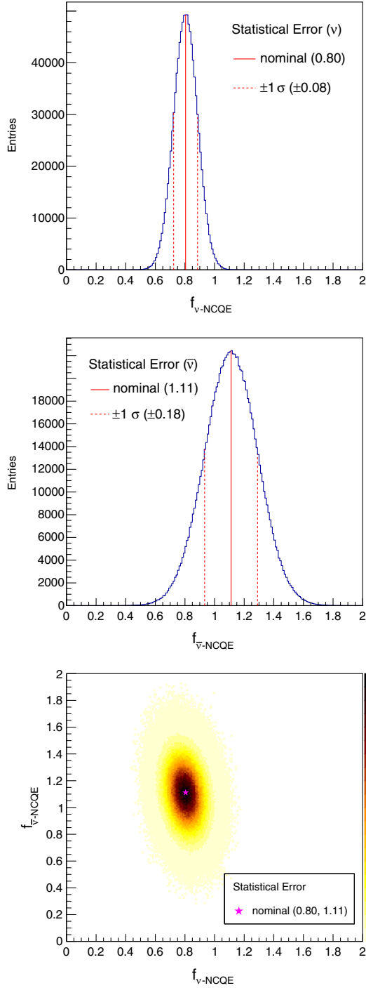
FIG. 10. Results of the pseudoexperiments on the scale factors when the numbers of events are varied based on the statistical uncertainties: f_{\nu\text{-NCQE}} = 0.80 \pm 0.08 and f_{\bar{\nu}\text{-NCQE}} = 1.11 \pm 0.18 .
