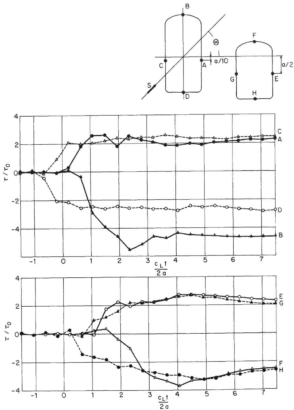
Fig.4.1.10.15 Transient hoop stresses around a pair of caverns; incident S wave.
