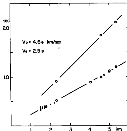
Fig. 4 Travel time of P and S waves from quarry blasts.
