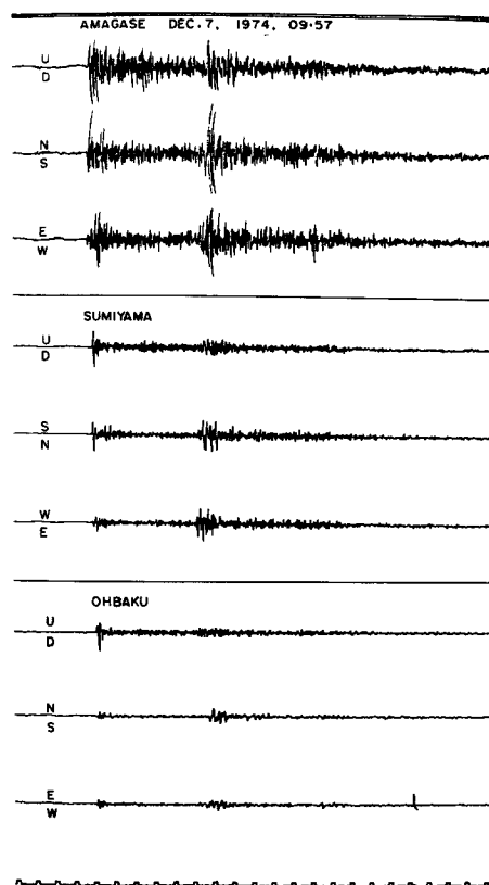
Fig. 2 Examples of local small earthquake recorded at three stations.
