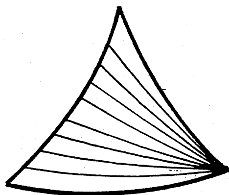
Fig. 2. Ordered "geodesic triangles".
