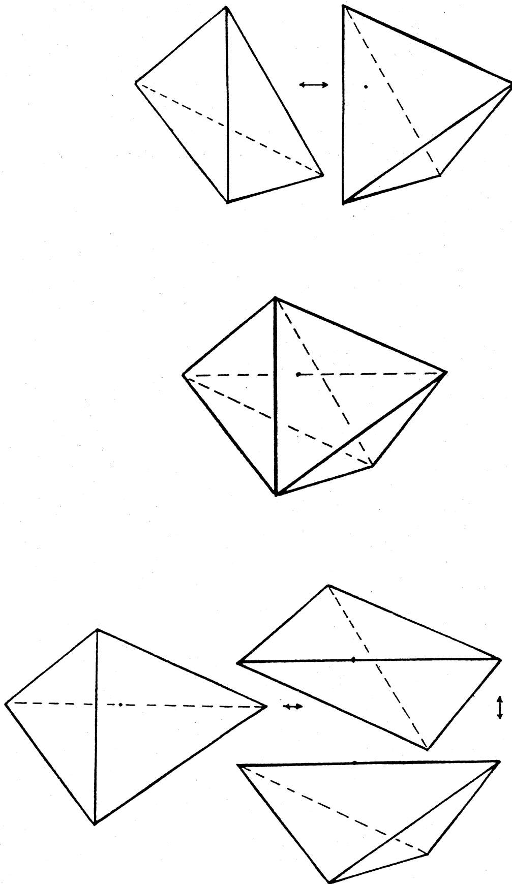
Fig. 1. Dividing a polytope in two different ways.
