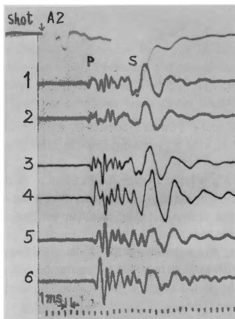
Fig. 3-3(a). Comparing responses for several kinds of installation (geophones : VP-3100 (natural frequency : 100 cps) ) trace 1-3 fixed with cement at the bottom of a drill hole (1.5m depth). trace 4 fixed with cement on the wall (rock) surface, trace 5 fixed with wooden wedge on the wall (rock) surface, trace 6 fixed with clay on the wall (rock) surface.
