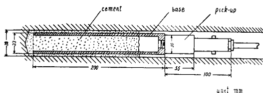
Fig. 3-3(b). Schematic explanation of installation condition of trace 1-3 in Fig. 3-3(a).
