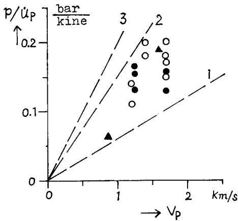
Fig. 3-9(a). Observed value of p/\dot{u}_P .
