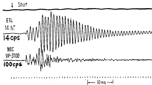
Fig. 3-1. A record comparing responses of two models of geophone for the same input signal. The upper trace shows predominant resonance of the second mode. (Cited from Kitsunezaki et al. [1960].)
