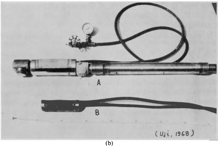
Fig. 4-8(b). Photographic view A S source B : geophone
