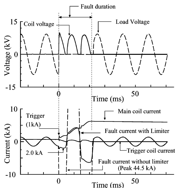
Fig. 5. Simulation result of a 6.6 kV, 1 kA system with 90° fault.
