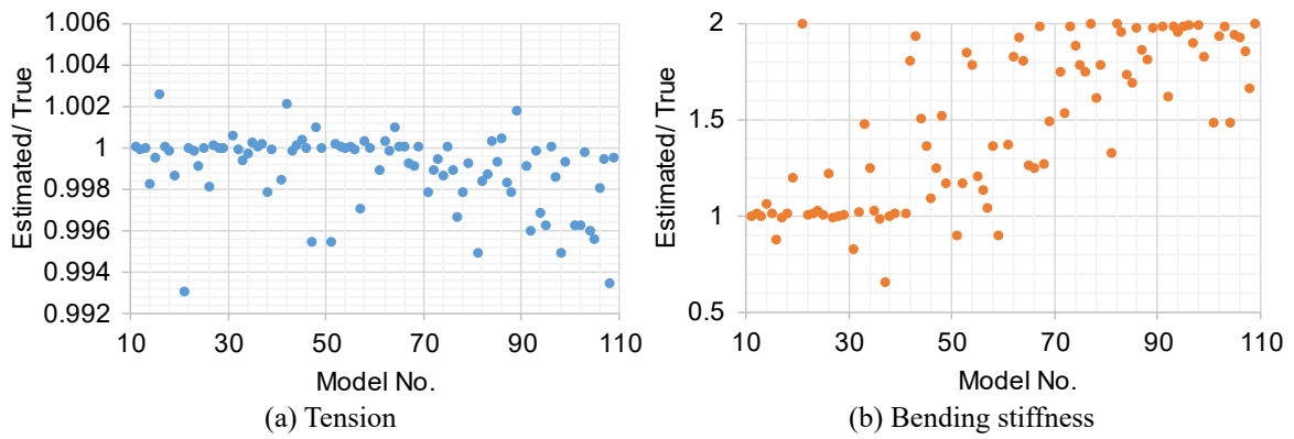
Fig. 3 Ratio of estimated value to true value for tension and bending stiffness for viscous shear damper when 1 st –5 th modes are used
