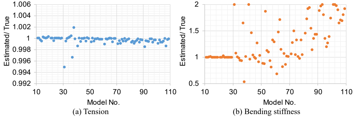
Fig. 5 Ratio of estimated value to true value for tension and bending stiffness for viscous shear damper when 1 st –7 th modes are used
