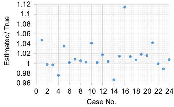
Fig. 7 Ratio of estimated tension to true tension by proposed method
