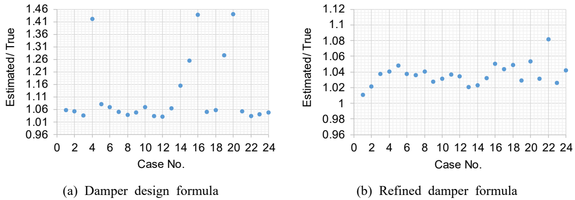
Fig. 8 Ratio of estimated tension to true tension by previously proposed method using different damper formulas
