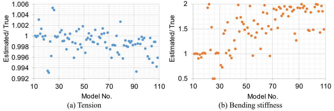
Fig. 2 Ratio of estimated value to true value of tension and bending stiffness for high-damping rubber damper when 1 st –5 th modes are used
