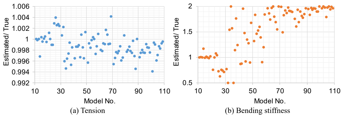
Fig. 4 Ratio of estimated value to true value for tension and bending stiffness for high-damping rubber damper when 1 st –7 th modes are used
