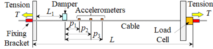
(a) Schematic diagram of test specimen, impact position, and measurement locations.
