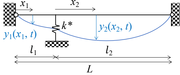
Fig. 1 Analytical model of cable with damper.
