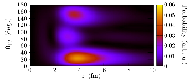
FIG. 3. Calculated [6] two-neutron probability densities for ^{19}\text{B} ( S_{2n} = 0.5 MeV, a_s = -50 fm). The density (weighted by 8\pi^2 r^4 \sin \theta_{12} ) is plotted as a function of neutron-core distance r_1 = r_2 = r and opening angle between the valence neutrons \theta_{12} . The density distribution shows substantial enhancement at small angles \theta_{12} \sim 25^\circ , indicating a dineutron correlation.
