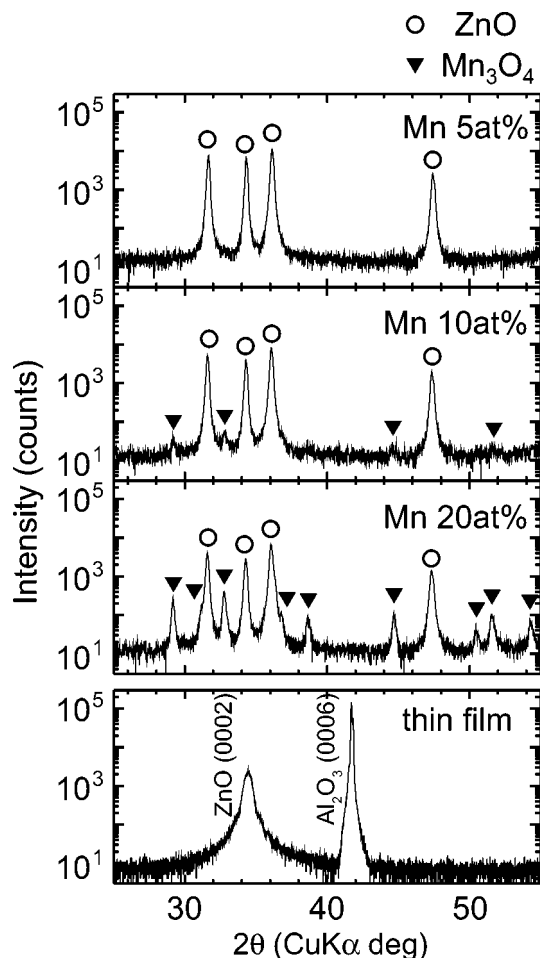
FIG. 1. XRD patterns of Mn-doped polycrystals with 5, 10, and 20 at.% Mn and a thin film with 5 at.% Mn.
