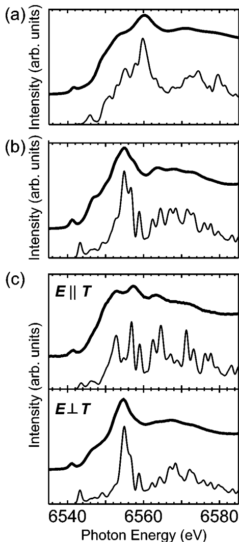
FIG. 3. Comparison of NEXAFS spectra between calculations and experiments for (a) \text{Mn}_3\text{O}_4 , Mn-doped ZnO, (b) polycrystal, and (c) thin film. \mathbf{E} and \mathbf{T} are the electric field vector and the vector perpendicular to the surface of the thin film, respectively. Thick and thin solid curves are experiments and calculations, respectively. Absolute transition energies of all theoretical spectra were shifted by -20 eV ( \Delta E/E=0.3\% ).
