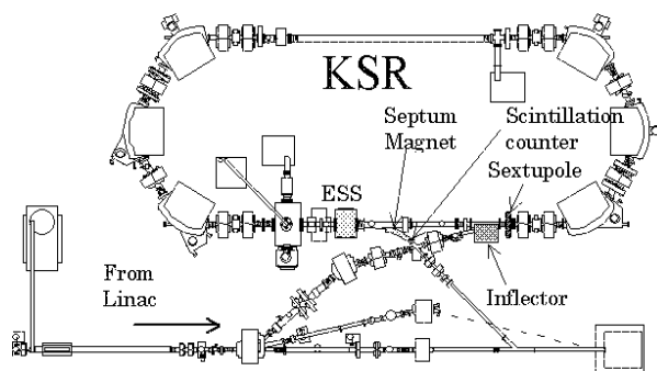
Figure 1. The layout of the KSR. Main devices for the beam injection and extraction are shown.
