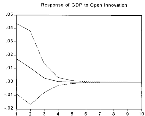
Fig. 4. Impulse response function: Seychelles
