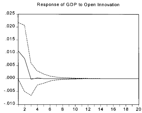
Fig. 2. Impulse response function: Madagascar
