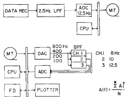
Fig. 3 Observational system of microseisms and frequency response of geophone
