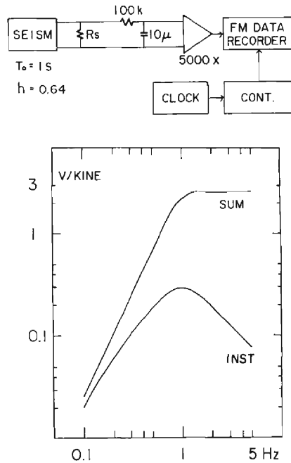
Fig. 3 Observational system of microseisms and frequency response of geophone
