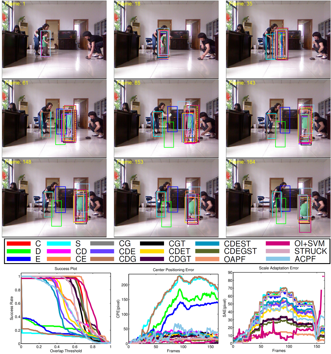
Figure A.4: Qualitative Analysis of sequence child_no1 , the ground truth is marked with yellow dashed line.
