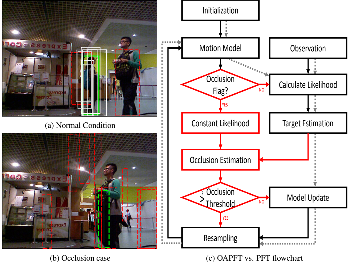
Figure 3.1: The dynamics of occlusion-aware particle filter ( OAPFT ) in normal conditions (a) and occluded conditions (b). Brighter boxes are more similar to the target and red boxes are marked as occluded. The green box is the estimated target location. The comparative flowchart of the PFT and the proposed OAPFT is illustrated in panel (c).
