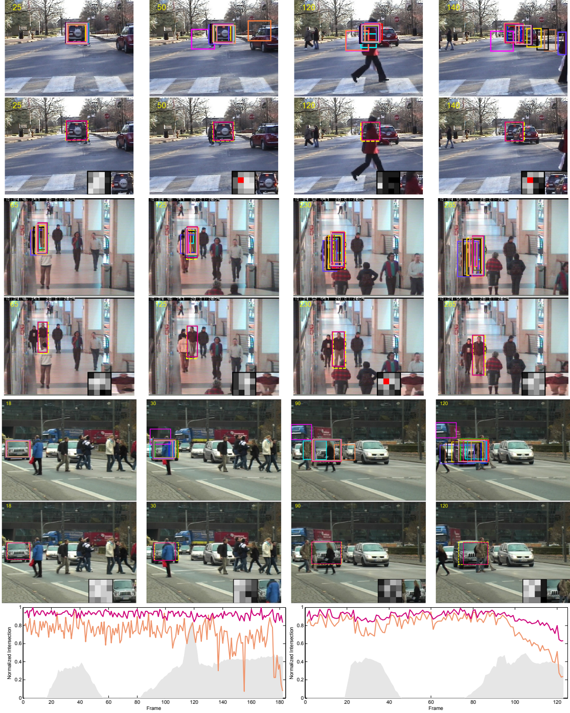
Figure 5.3: The tracking results of our algorithm on the campus ( top ), CAVIAR ( middle ) and TUD-Crossing ( bottom ) sequences. Ground truth is illustrated by yellow dotted line, while three best trackers ( LIAPG-OPM , LIT-OPM , and LIT-OR and two worst trackers ( OAB and BSB ) for these scenarios are depicted on the frames. Isolated and noisy occlusion regions have been successfully detected as it is illustrated by the occlusion masks. The localization error of LIAPG and LIAPG-OPM is illustrated on the lower panel, while the shaded area indicates the extent of the occlusion.
