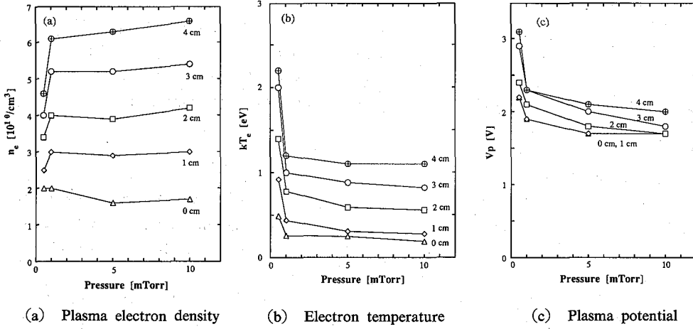
Fig. 6. The dependence of plasma parameters on the H_2 gas pressure.
