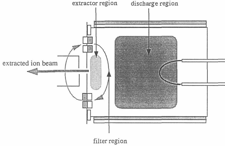
Fig. 2. The magnetic cusp field configuration near the PE.
