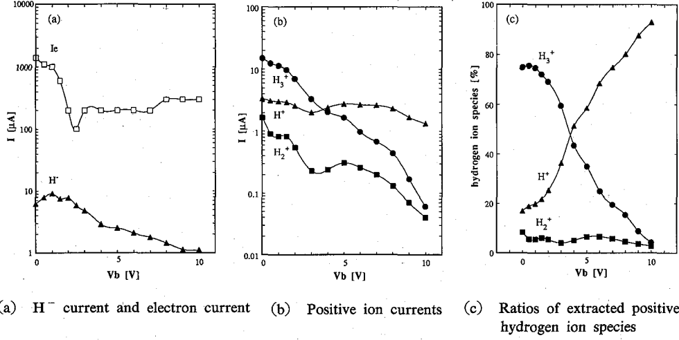
Fig. 8. The dependence of extracted beam currents upon the PE bias voltage.
