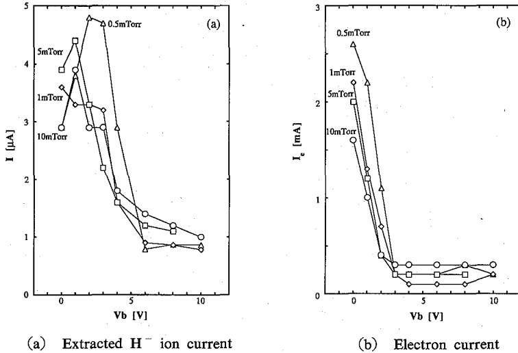
Fig. 7. The extracted beam currents as a function of the PE bias voltage for several H_2 gas pressures.
