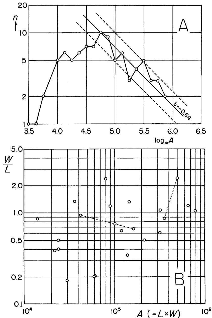
Fig. 5 Frequency-Magnitude (area) relationship (A), and Form ratio-Magnitude relationship (B) for landslides in Nishi-Totsukawa area, where L ; length, W ; width, A (=L \times W) ; area, and n number of landslides, respectively.
