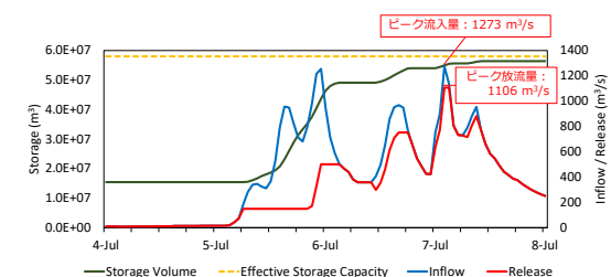
Fig. 9 Simulation results of operation of the Hyogoshi Reservoir for the generated hypothetical flood event.
