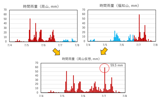
Fig. 8 Example of the method applied to generate hypothetical hyetograph for each rain gauge around the Hyogoshi Reservoir.
