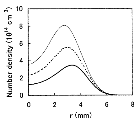
FIG. 11. Number density of sodium ions at three axial positions as a function of radial distance at the maximum current.
