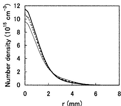
FIG. 8. Number density of electrons at three axial positions as a function of radial distance at the maximum current.
