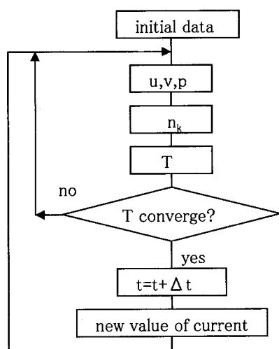
FIG. 2. Flow chart of numerical calculations as a function of time. Time t is advanced by \Delta t after temperature T converges.
