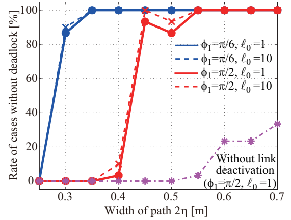
Fig. 8. Rate of cases without deadlock for M = 1 and \phi_1 = \frac{\pi}{6}, \frac{\pi}{2} .
