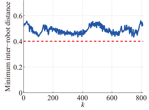
Fig. 13. Minimum inter-robot distance (experiment).
