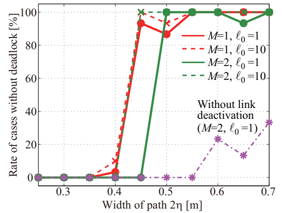
Fig. 9. Rate of cases without deadlock for M = 1, 2 and \phi_1 = \frac{\pi}{2} .
