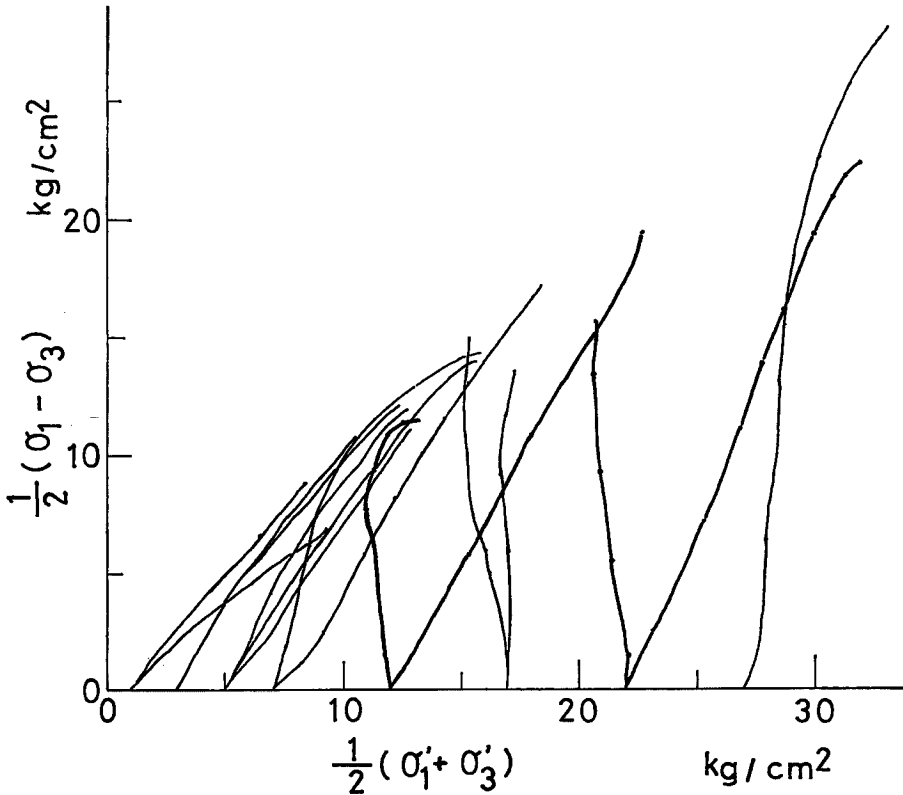
Fig. 8 Stress path for consolidated-undrained test under initial back pressure u_b = 3.0 \text{ kg/cm}^2 .
