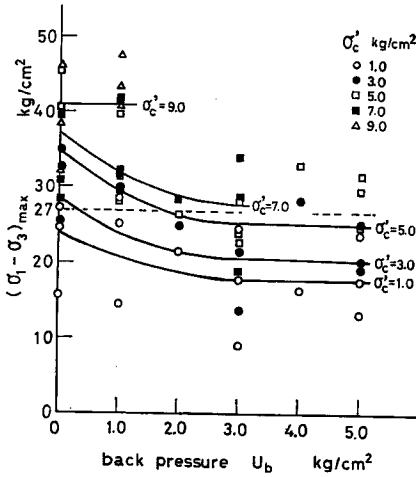
Fig. 6 Influence of initial back pressure on maximum deviator stress in CU-test; Average value of strength under undrained test is 27.0 \text{ kg/cm}^2 .
