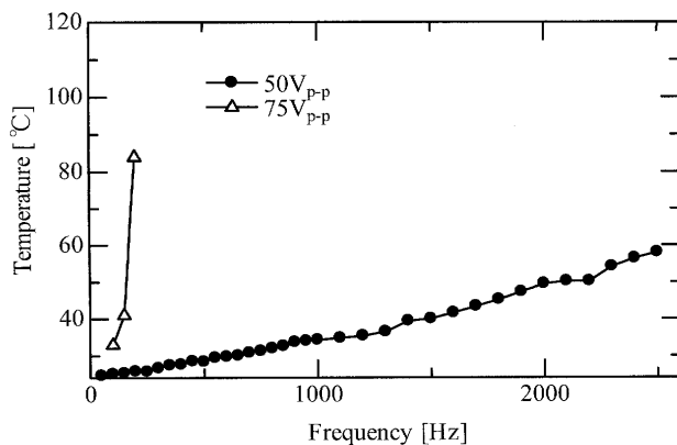
Fig. 5 Relationship between applied frequency and temperature of the piezoelectric actuator.
