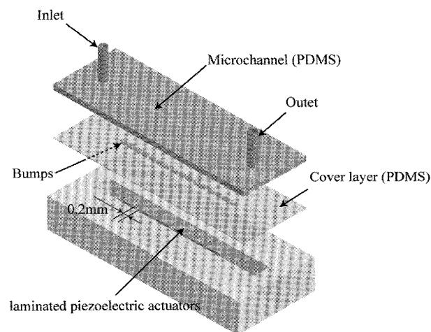
Fig. 2 Exploded view of traveling wave micropump.
