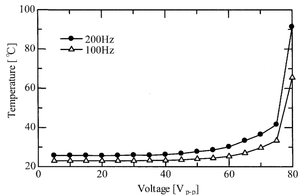
Fig. 6 Relationship between applied voltage and temperature of the piezoelectric actuator.
