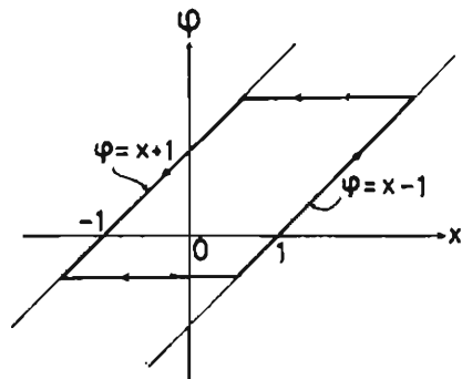
Fig. 2. Backlash characteristic.
