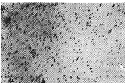
Fig. 8 Al-Zn-Mg Alloy aged 5 hr. at 250°C
