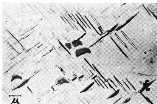
Fig. 4 Al-Cu Alloy aged 2½ hr. at 300°C
