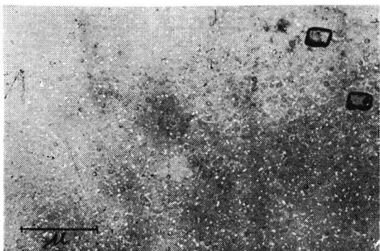
Fig. 9 Al-Zn-Mg-Cu Alloy aged 30 hr. at 200°C
