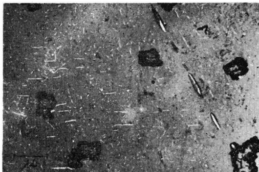
Fig. 6 Al-Cu-Mg Alloy aged 30 hr. at 200°C and furthermore 30 hr. at 250°C
