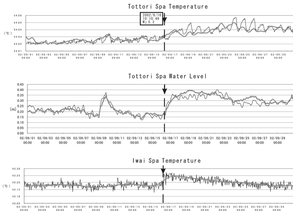
Fig.8 An example record section of subsurface water temperatures.
