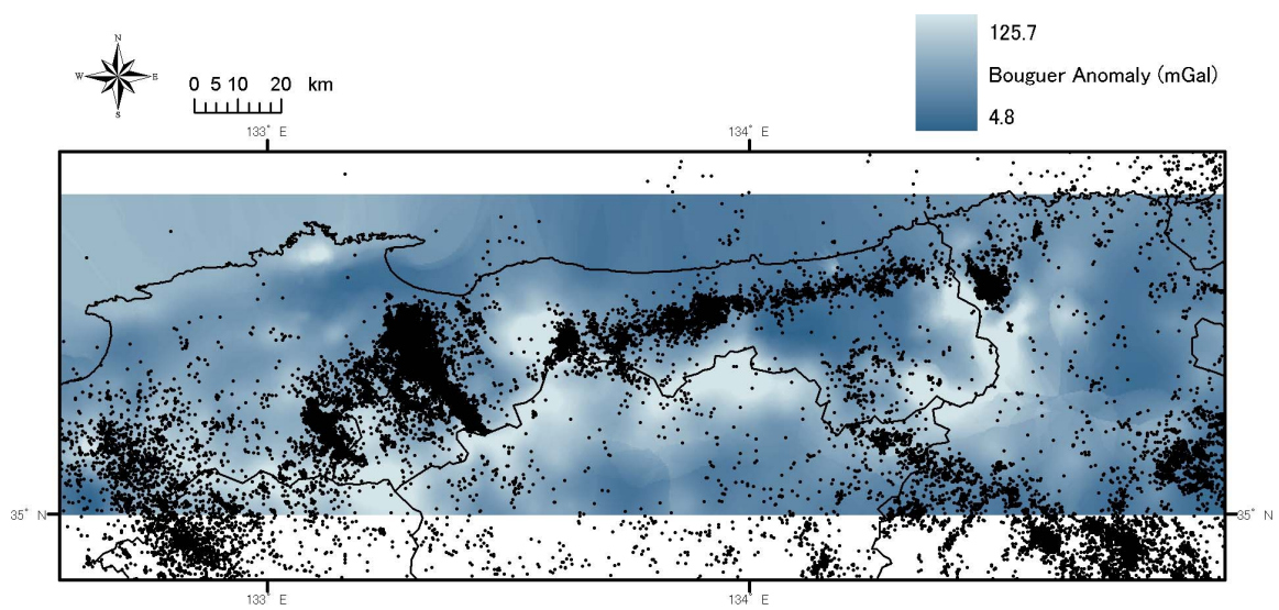
Fig.11 Overlaid map of the hypocentral distribution and the gravity anomalies. The gravity anomalies are calculated with an assumed density of 0.4\text{g/m}^3 .
