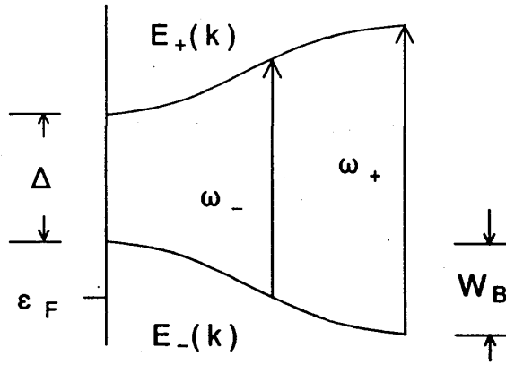
Fig. 1. The band scheme of a free two-band model at T = 0 with its characteristic parameters and energies
