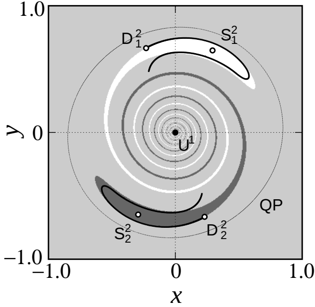
Fig. 4. Basin structure and approximate expression for discrete dynamical system P_0^\varepsilon associated with non-autonomous system (23). The fixed point U^1 is completely unstable, that is, source, and S(\text{or } D)_i^2 ( i = 1, 2 ) stand for the completely stable (or directly unstable) 2-periodic points.
